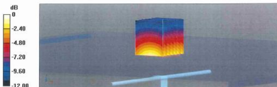
0 dB = 3.64 W/kg = 5.61 dBW/kg
