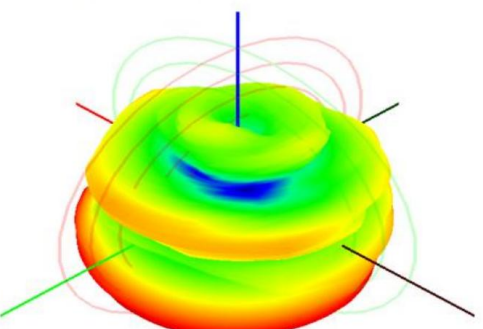
5350.0MHz H+V, Eff. 49.21%
