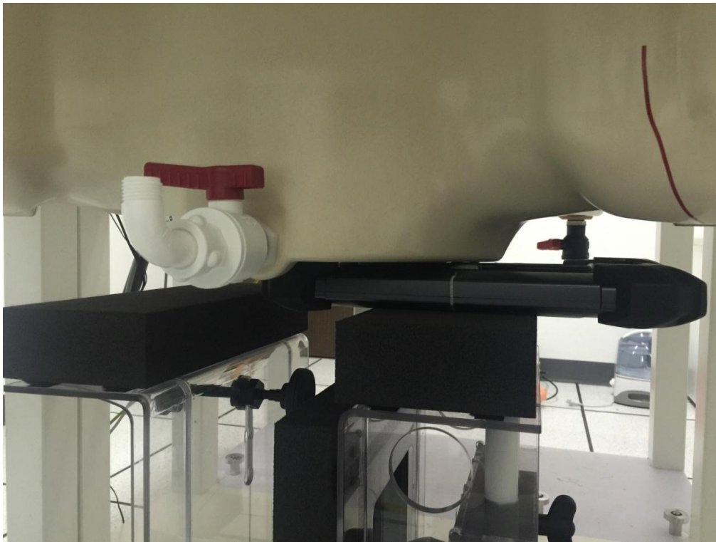
2.4G Edge_2 with Gap 0mm
