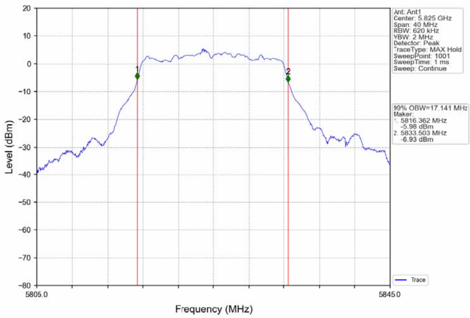
802.11a_HCH_5825MHz_Ant1_NTNV
