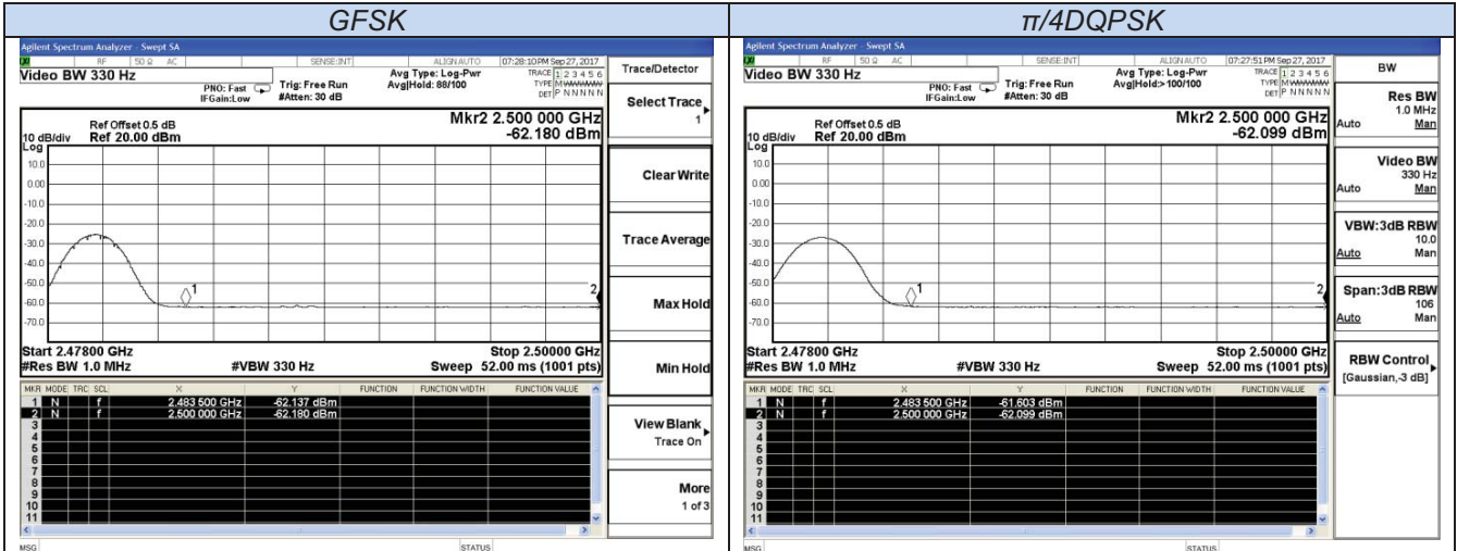
Channel 78 / 2480 MHz – Non-Hopping – Average
