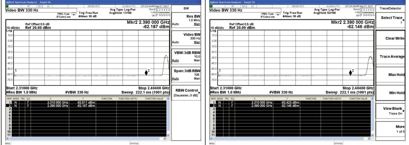
Channel 0 / 2402 MHz – Non-Hopping – Average
