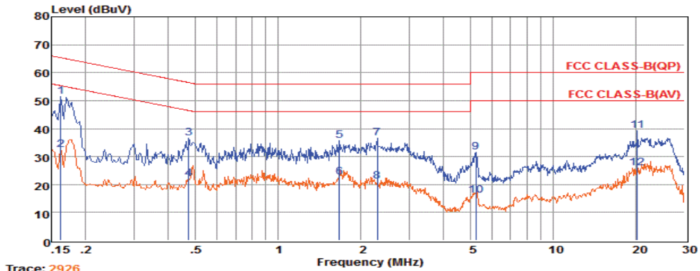
Trace: 2926 Pol: NEUTRAL
