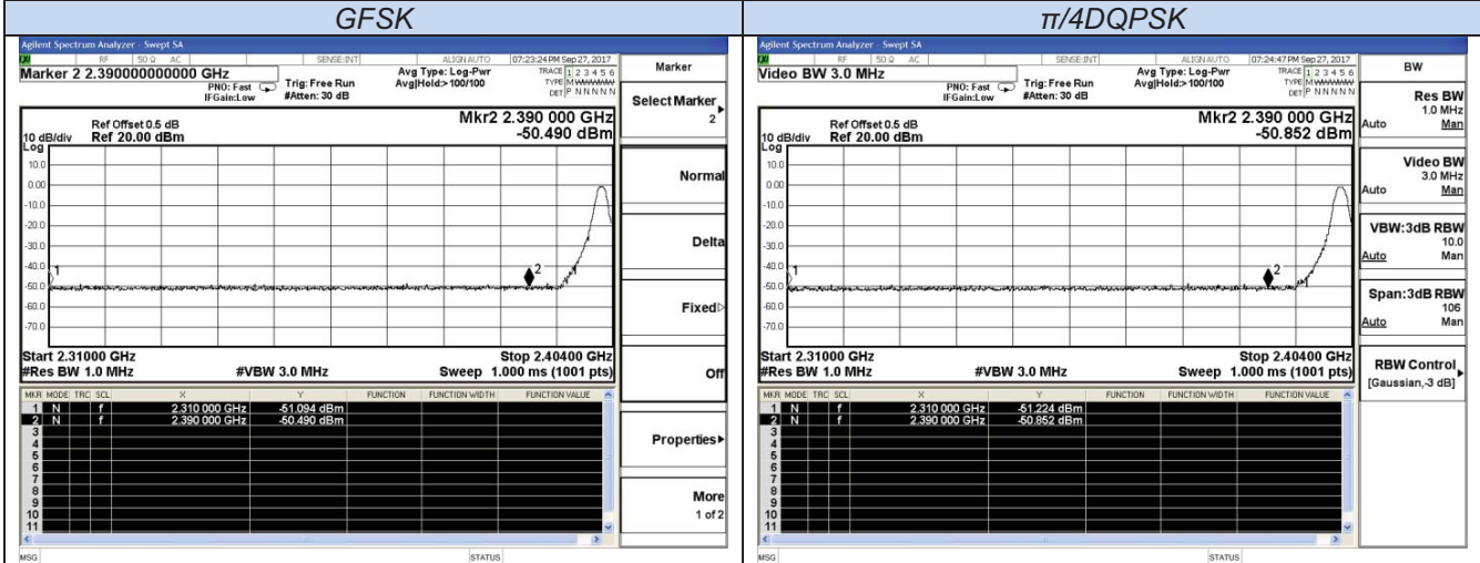
Channel 0 / 2402 MHz – Non-Hopping – Peak
