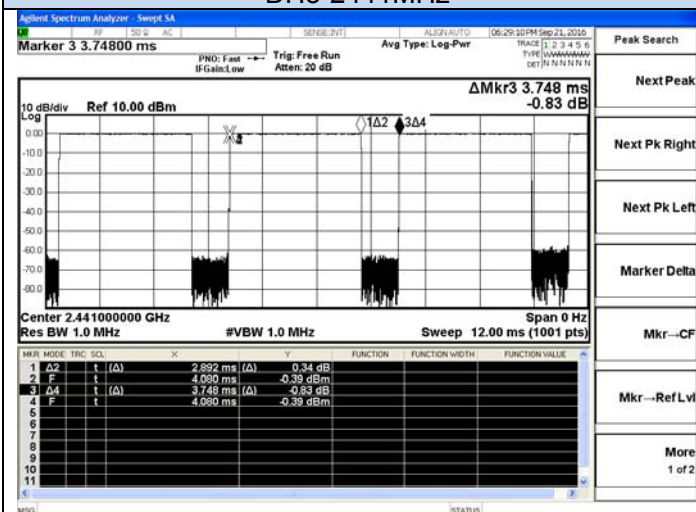
DH5-2441MHz
