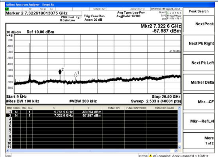
2DH1-Middle channel
