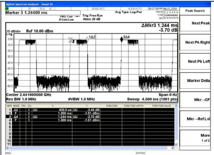
2DH1-2441MHz
