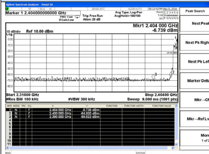
Hopping On-8-DPSK-Low channel
