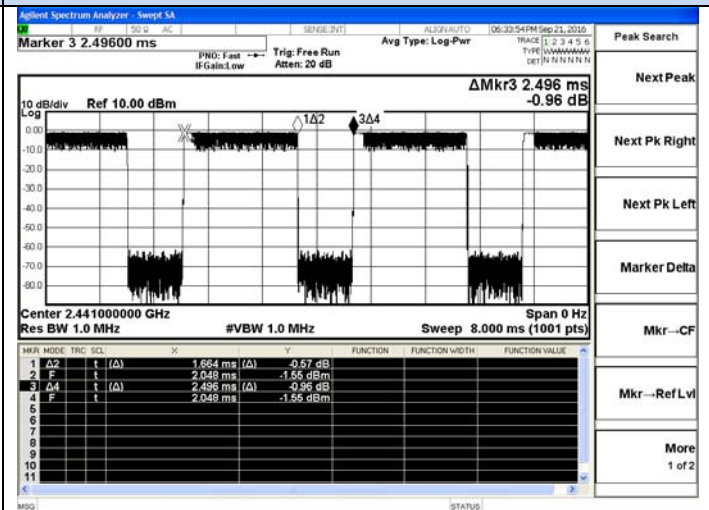
2DH3-2441MHz
