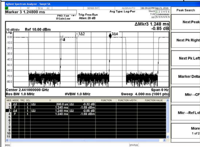
DH1-2441MHz
