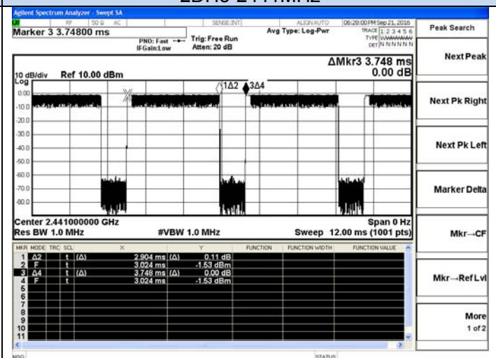
2DH5-2441MHz
