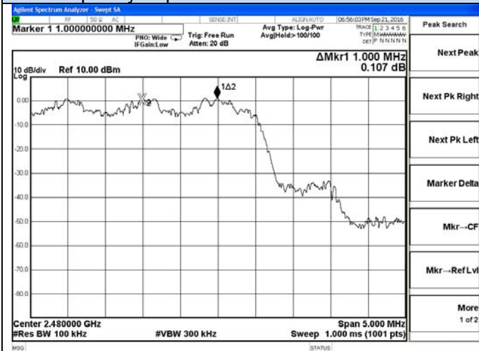
Frequency Separation 8-DPSK-High channel
