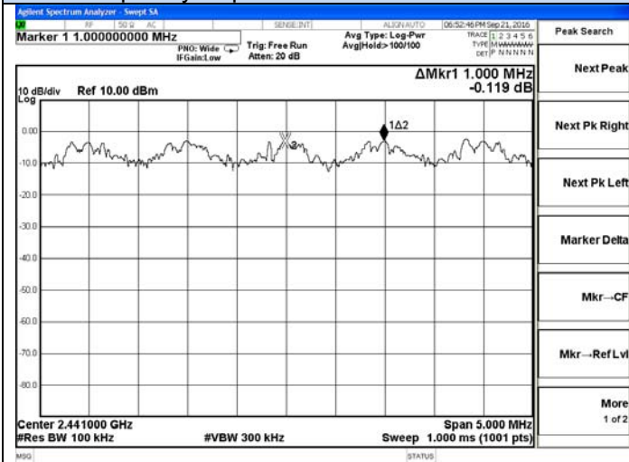
Frequency Separation 8-DPSK-Middle channel
