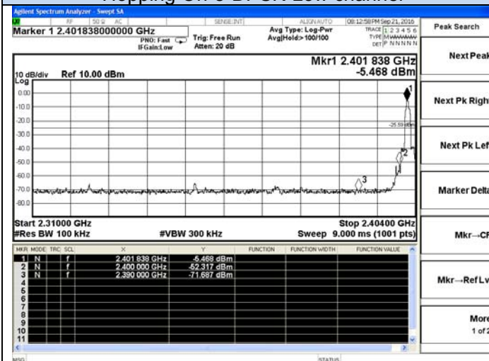
Hopping Off-8-DPSK-Low channel
