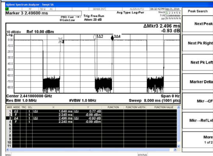
DH3-2441MHz
