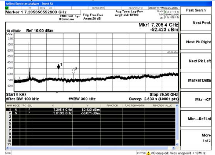
2DH1-Low channel
