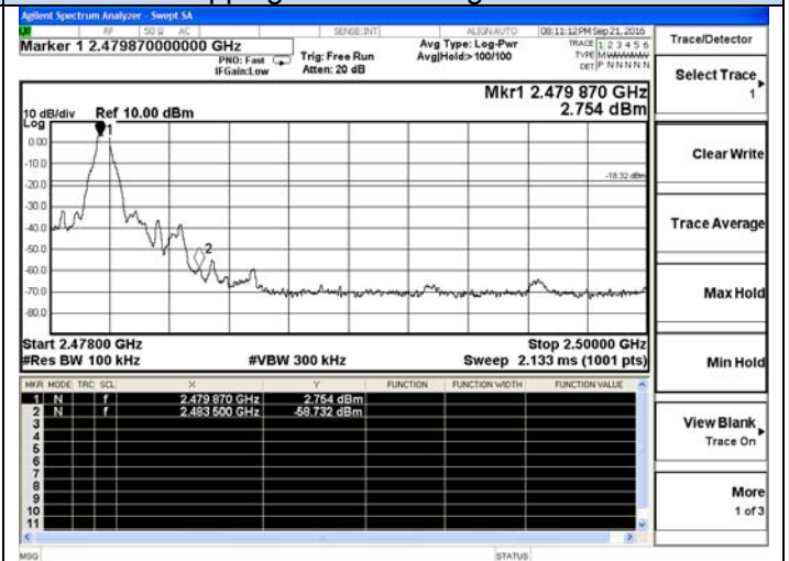
Hopping Off-GFSK-High channel
