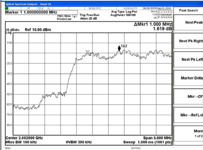
Frequency Separation 8-DPSK-Low channel
