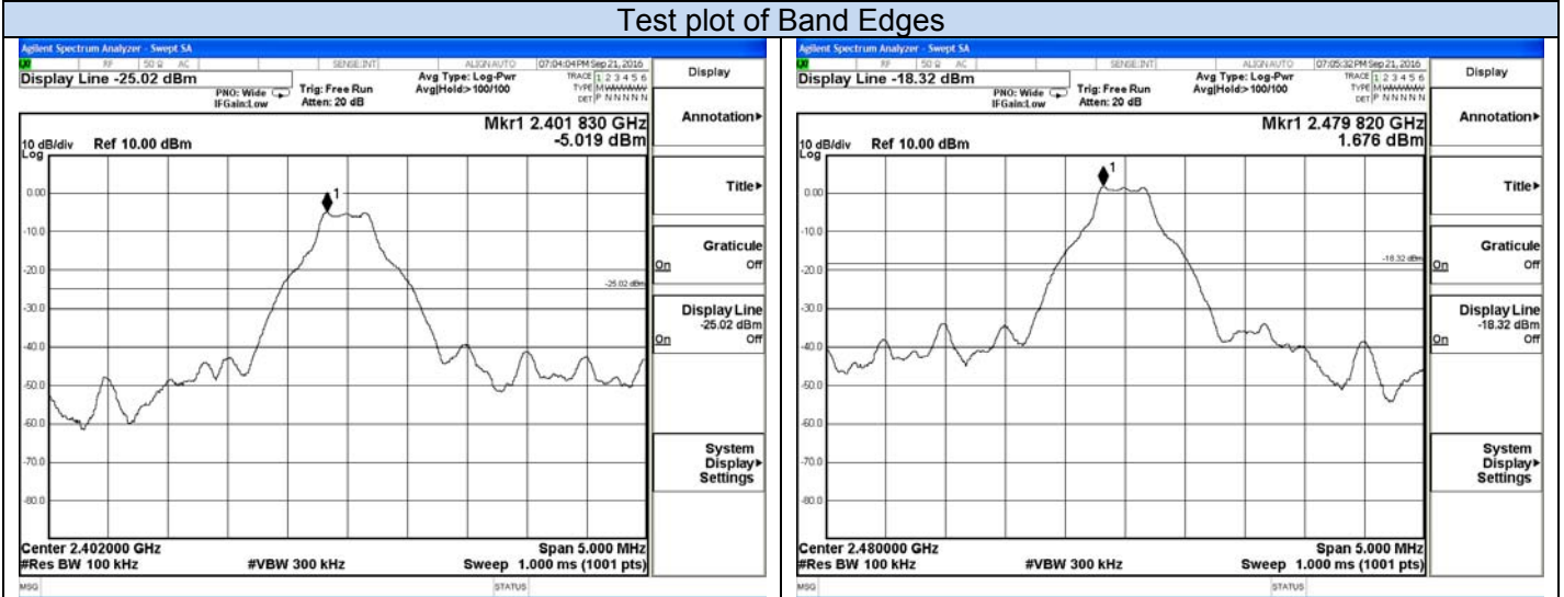
Reference of GFSK-Low channel
