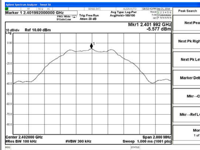
BT LE-Low channel Reference
