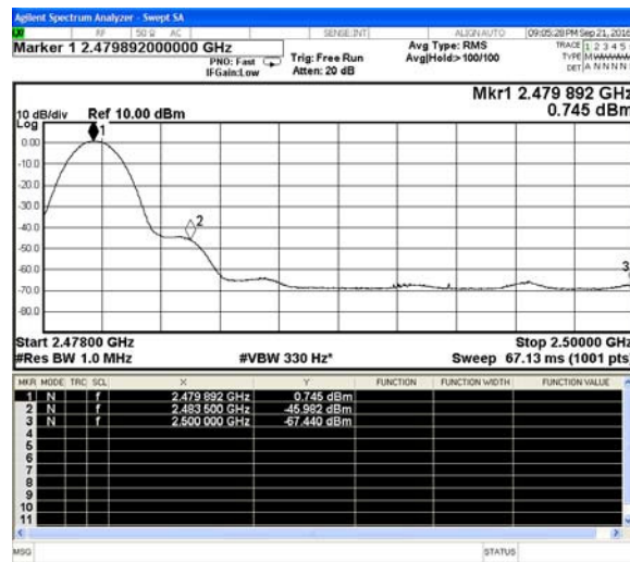
BT LE-High channel(Average)
