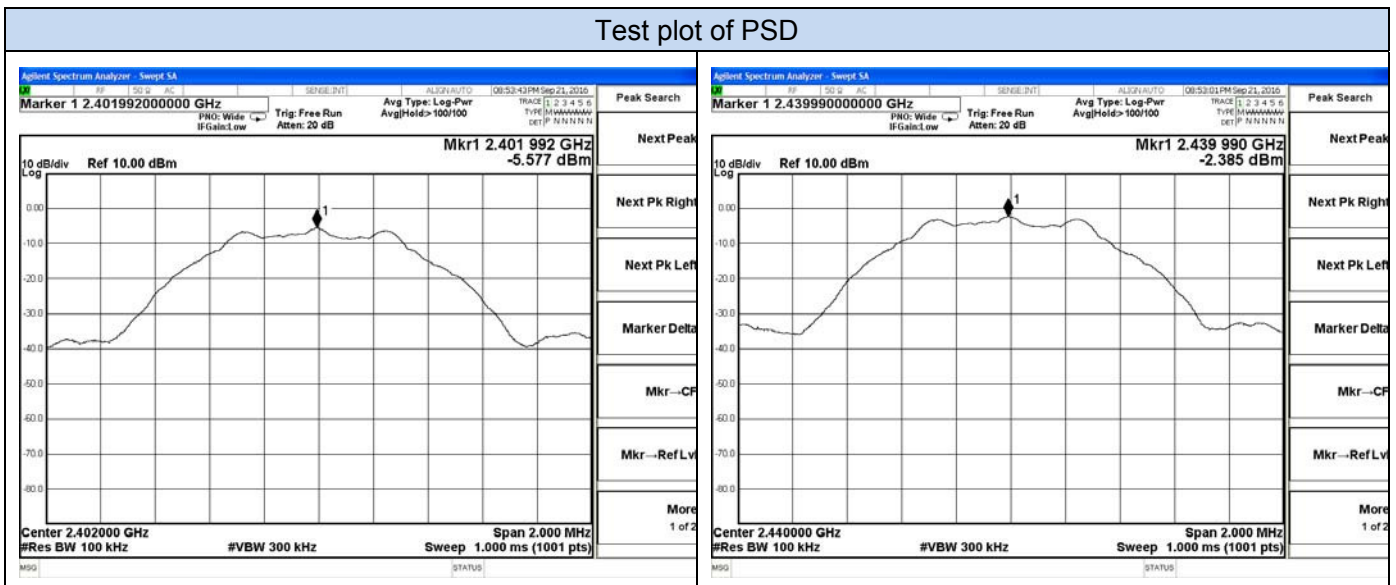
BT LE-Low channel
