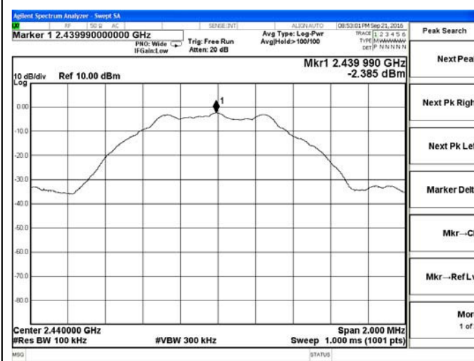
BT LE-Middle channel Reference
