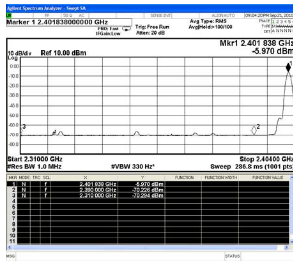
BT LE-Low channel(Average)
