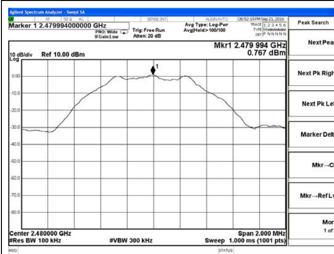
BT LE-High channel Reference
