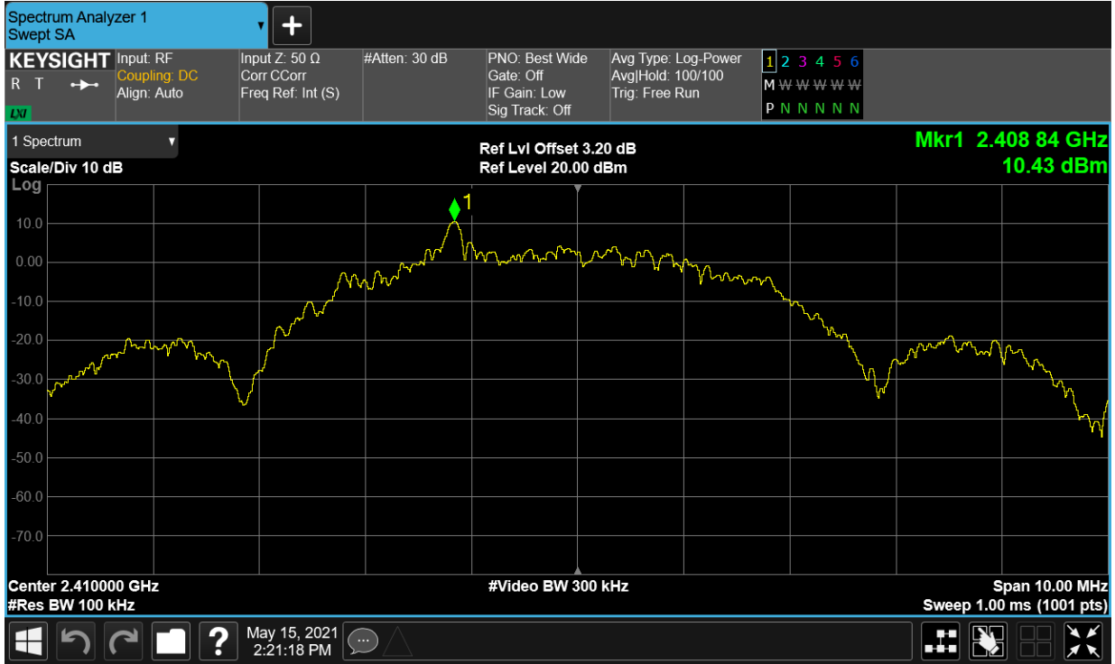
Band Edge NVNT SRD 2410MHz Ant1 No-Hopping Emission
