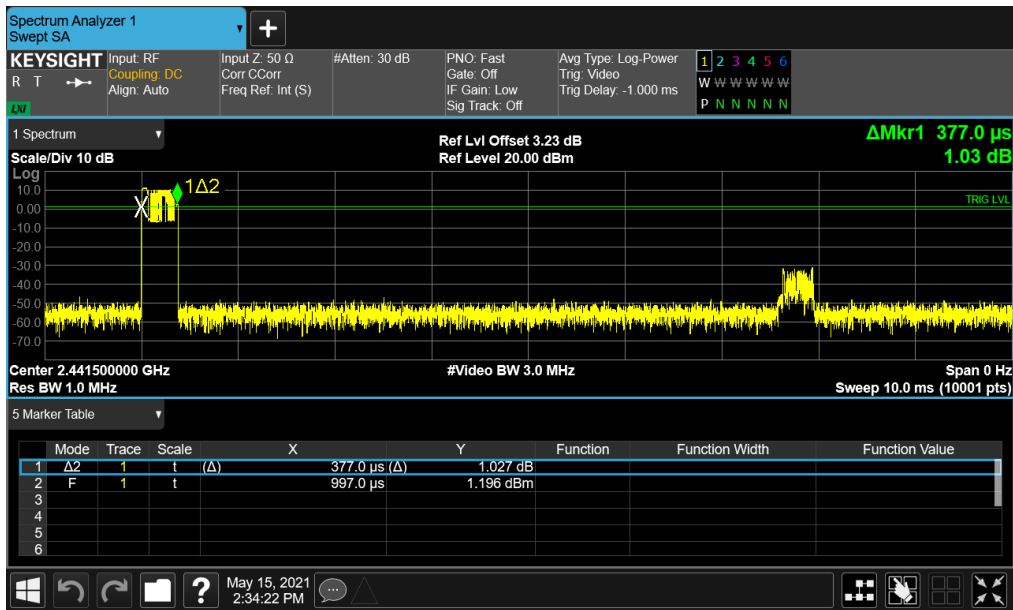
Dwell NVNT SRD 2441.5MHz Ant1
