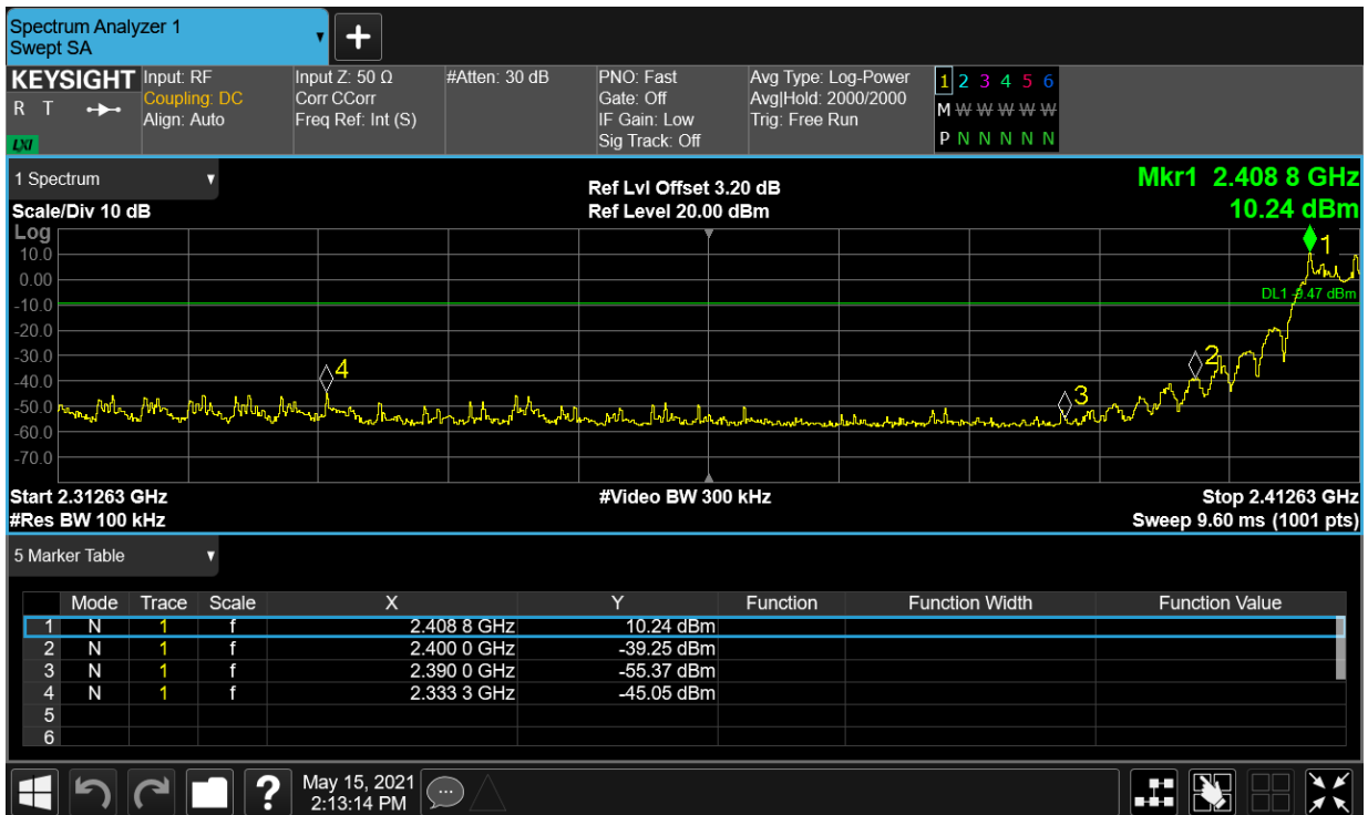
Band Edge(Hopping) NVNT SRD 2410MHz Ant1 Hopping Emission
