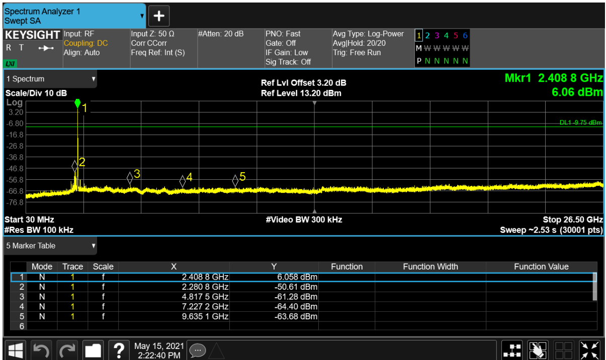
Tx. Spurious NVNT SRD 2410MHz Ant1 Emission
