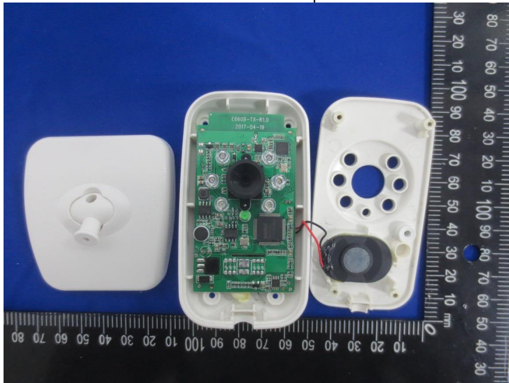
E600T model internal photos
