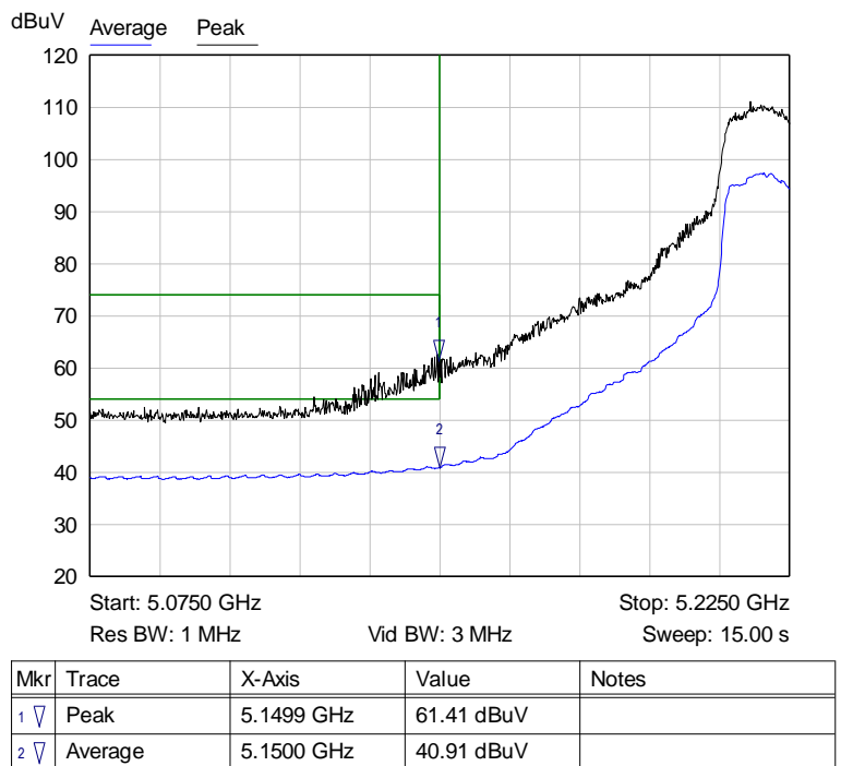
Graph 51: Antenna 1 – Channel 44 Band Edge at the Restricted Band Plot – Setting 20
