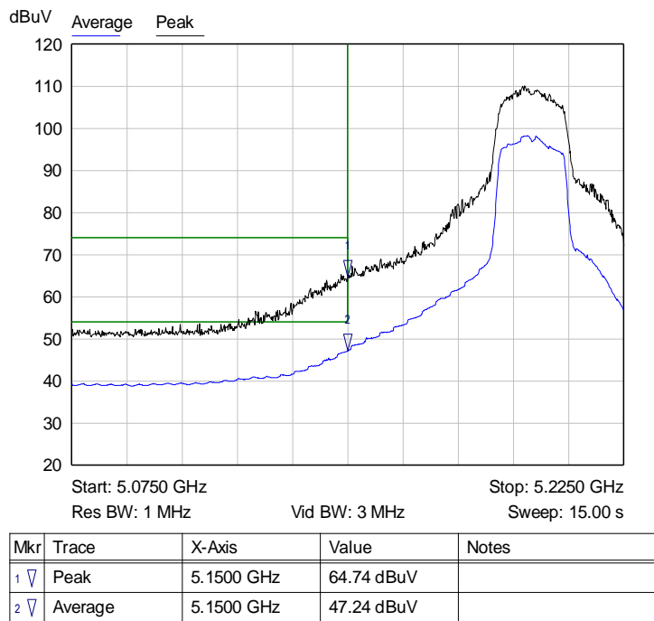
Graph 53: Antenna 0 – Channel 40 Band Edge at the Restricted Band Plot – Setting 18
