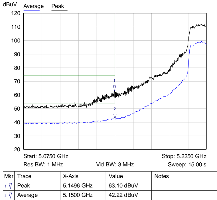
Graph 42: Antenna 0 – Channel 44 Band Edge at the Restricted Band Plot – Setting 20
