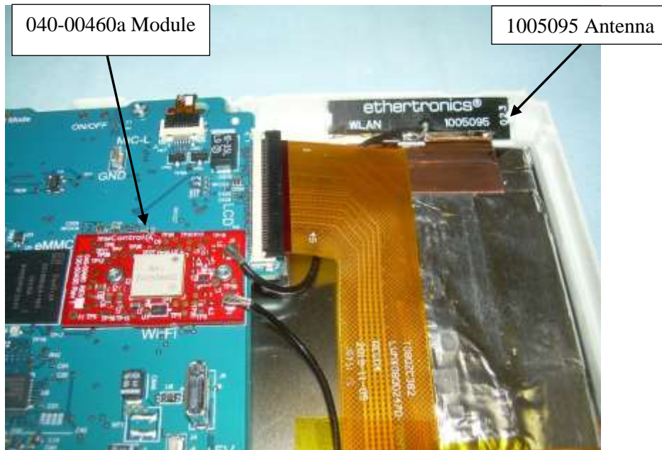
Photograph 25: 040-00460a Installed in C4-T4IW8-XX with 1005095 Antennas Installed
