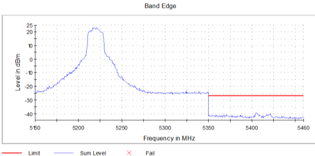
Graph 15: Antenna 0 – Upper Band Edge Channel 44 Transmitting (5220MHz) - Setting 20
