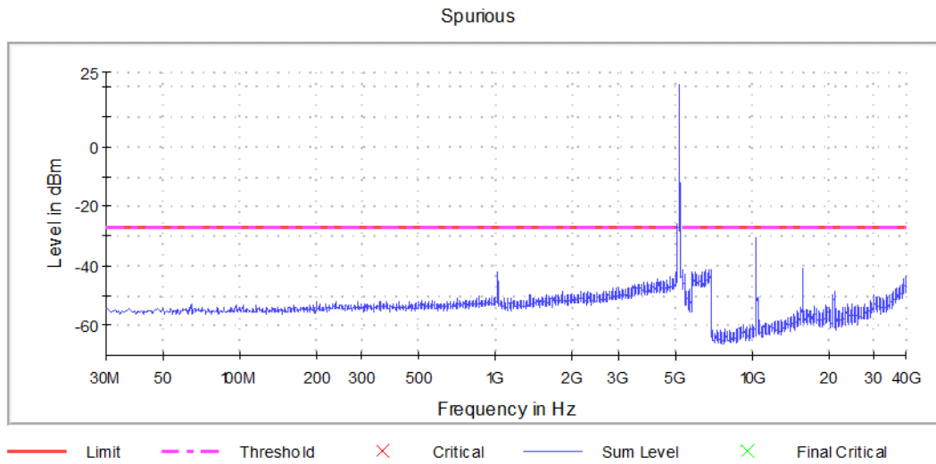
Graph 28: Antenna 0 – Spurious Emissions Channel 44 Transmitting (5220MHz) – Setting 20
