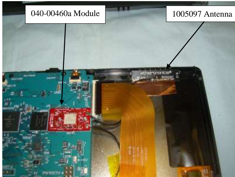
Photograph 22: 040-00460a Installed in C4-T4IW10-XX with 1005097 Antenna Installed
