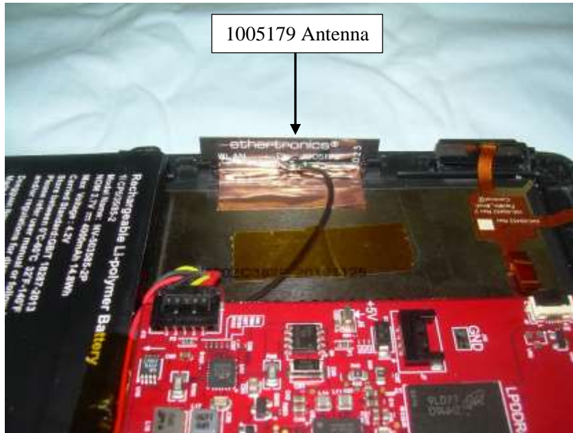
Photograph 20: 040-00460a Installed in C4-T4T8-XX with 1005179 Antenna Installed
