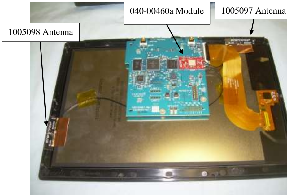
Photograph 21: 040-00460a Installed in C4-T4IW10-XX with 1005097 and 1005098 Antennas Installed
