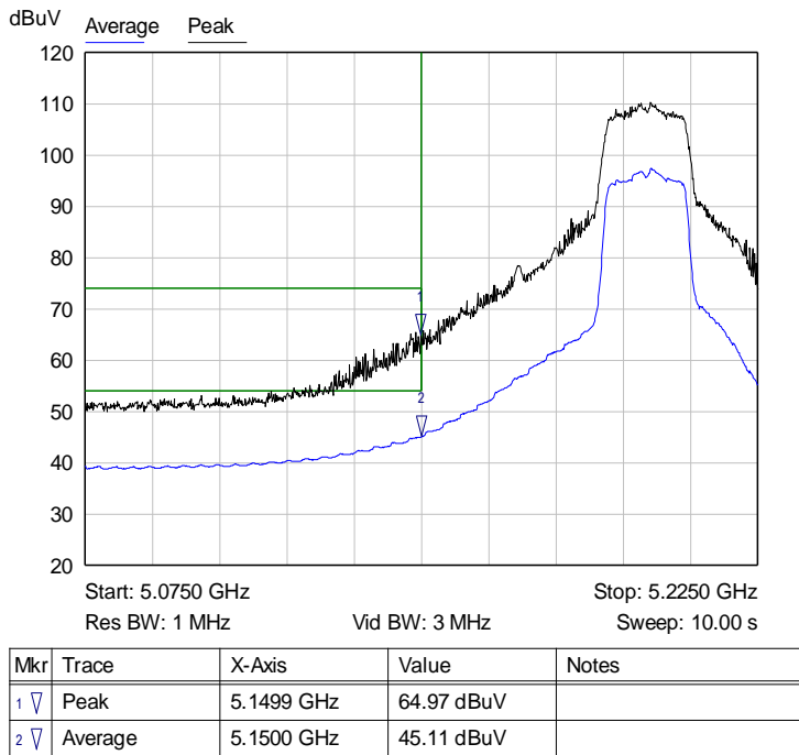
Graph 44: Antenna 1 – Channel 40 Band Edge at the Restricted Band Plot – Setting 18
