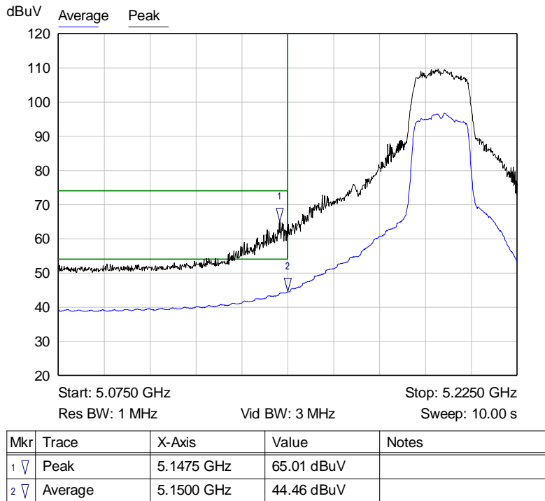
Graph 38: Antenna 1 – Channel 40 Band Edge at the Restricted Band Plot – Setting 18
