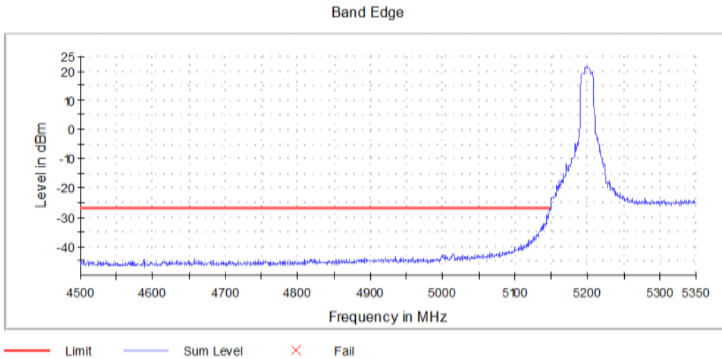
Graph 12: Antenna 0 – Lower Band Edge Channel 40 Transmitting (5200MHz) - Setting 18
