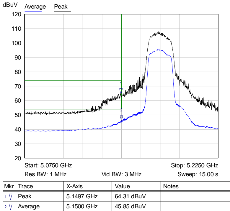
Graph 52: Antenna 0 – Channel 36 Band Edge at the Restricted Band Plot – Setting 13
