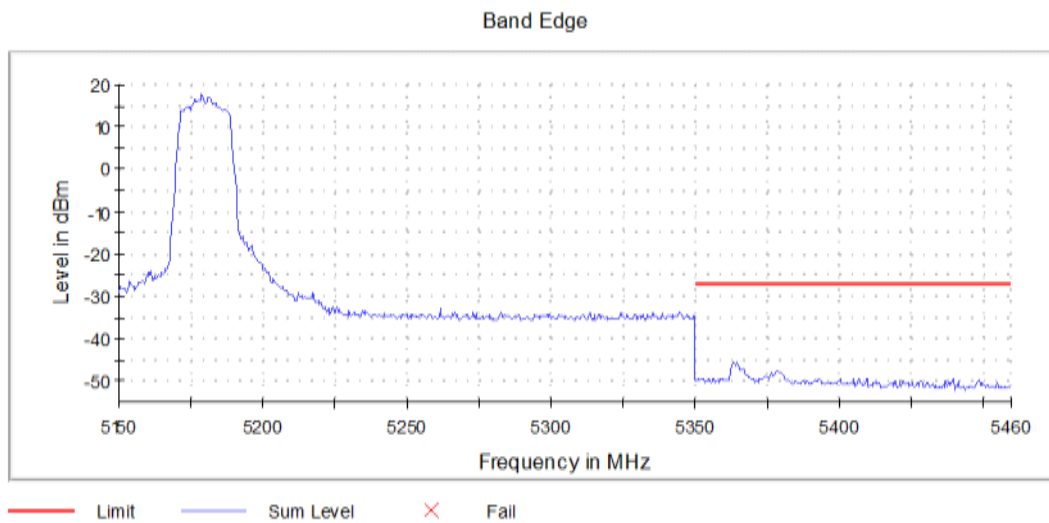
Graph 11: Antenna 0 – Upper Band Edge Channel 36 Transmitting (5180MHz) - Setting 13
