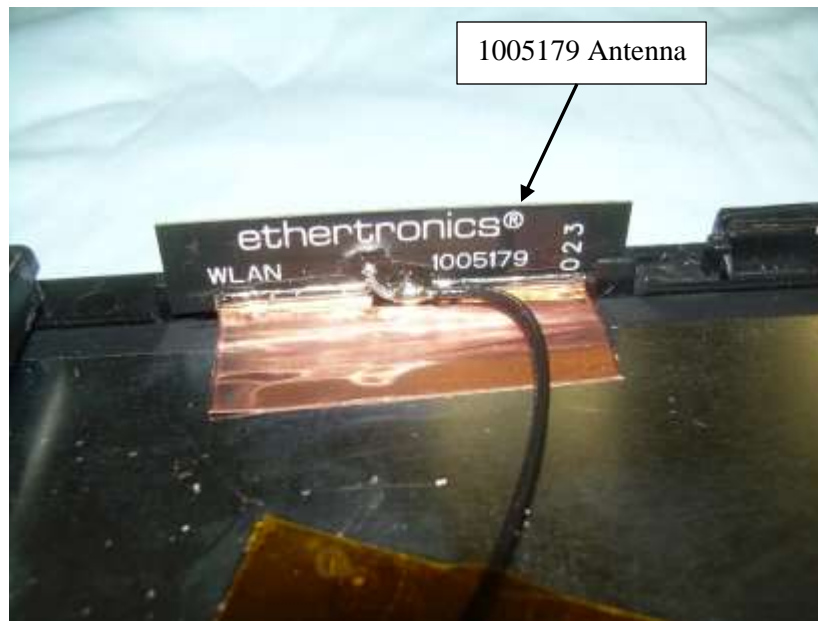
Photograph 17: 040-00460a Installed in C4-T4T10-xxwith 1005179 Antennas Installed
