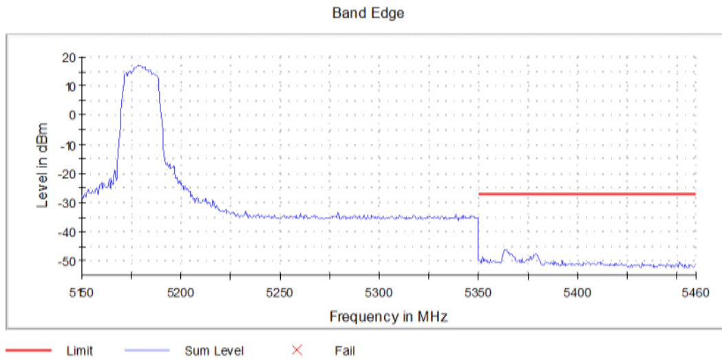
Graph 19: Antenna 1 – Upper Band Edge Channel 36 Transmitting (5180MHz) - Setting 13
