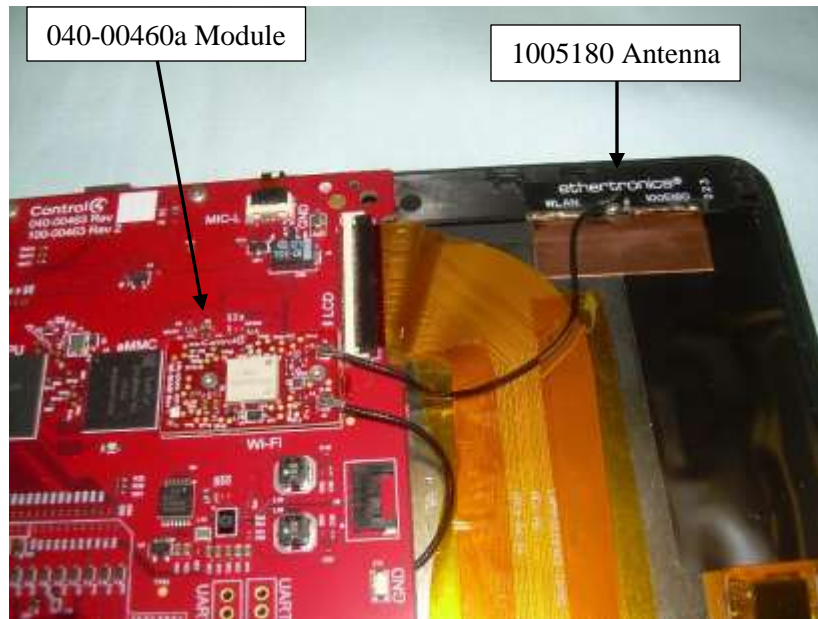
Photograph 16: 040-00460a Installed in C4-T4T10-xxwith 1005180 Antennas Installed
