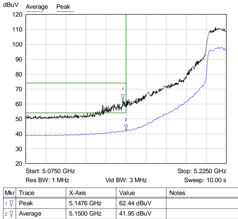
Graph 48: Antenna 0 – Channel 44 Band Edge at the Restricted Band Plot – Setting 20
