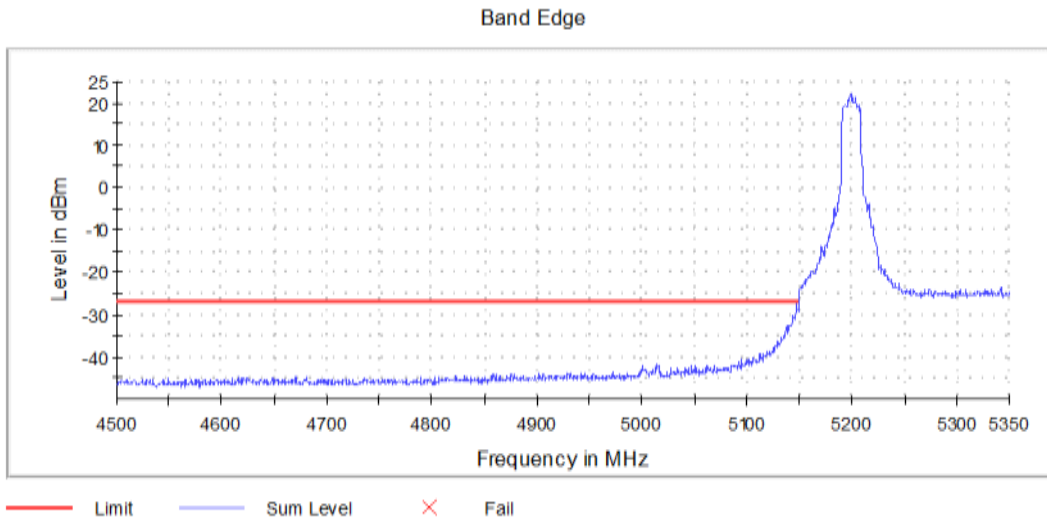
Graph 20: Antenna 1 – Lower Band Edge Channel 40 Transmitting (5200MHz) - Setting 18
