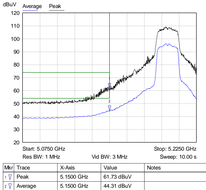
Graph 35: Antenna 0 – Channel 40 Band Edge at the Restricted Band Plot – Setting 18
