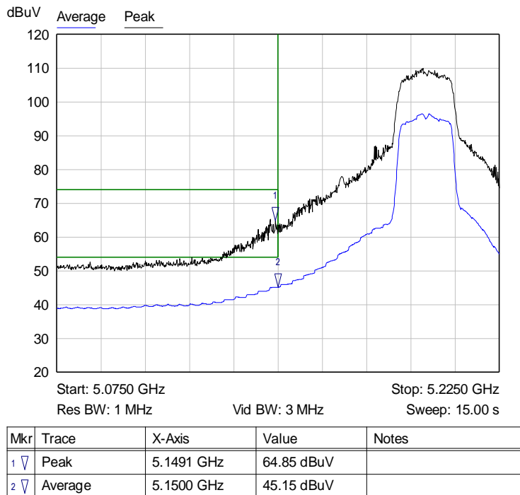
Graph 41: Antenna 0 – Channel 40 Band Edge at the Restricted Band Plot – Setting 18
