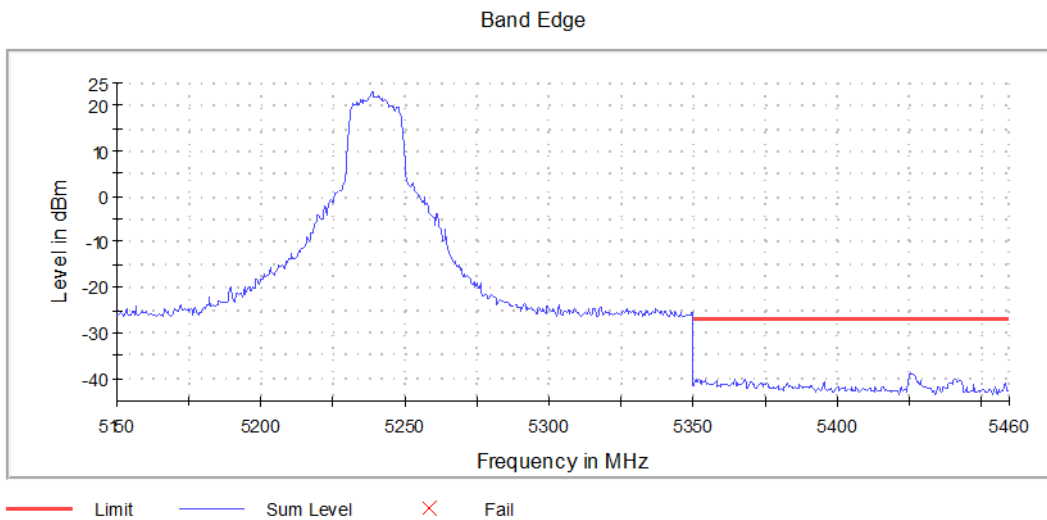
Graph 25: Antenna 1 – Upper Band Edge Channel 48 Transmitting (5240MHz) - Setting 20
