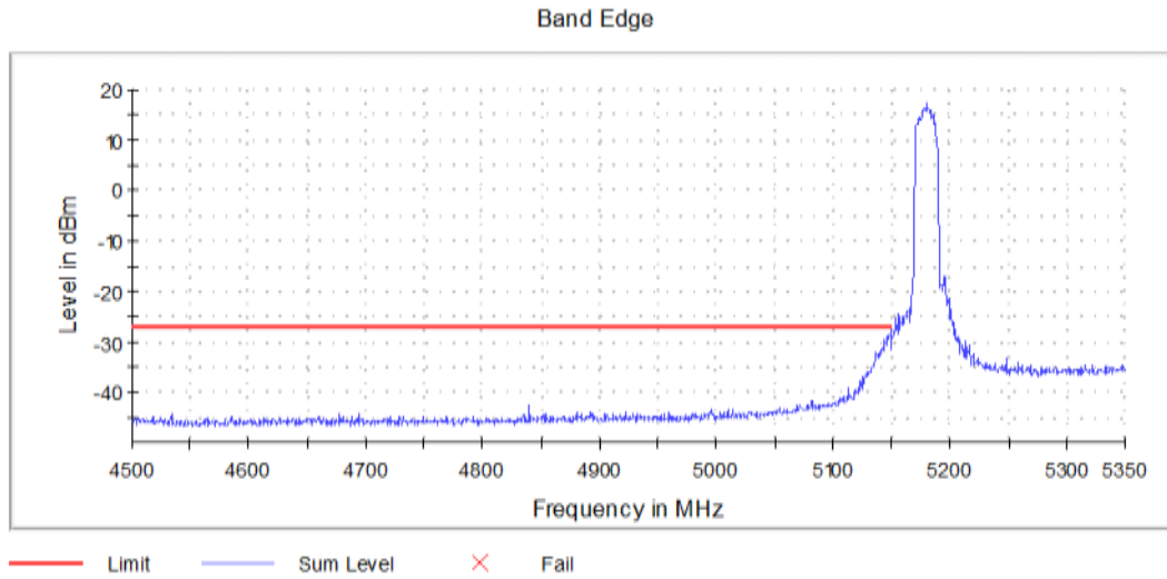
Graph 18: Antenna 1 – Lower Band Edge Channel 36 Transmitting (5180MHz) - Setting 13
