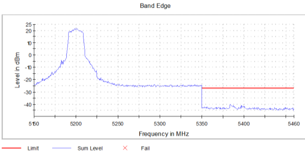
Graph 21: Antenna 1 – Upper Band Edge Channel 40 Transmitting (5200MHz) - Setting 18
