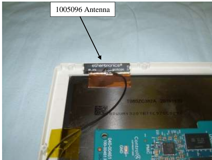
Photograph 26: 040-00460a Installed in C4-T4IW8-XX with 1005096 Antenna Installed
