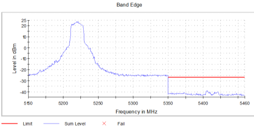
Graph 23: Antenna 1 – Upper Band Edge Channel 44 Transmitting (5220MHz) - Setting 20
