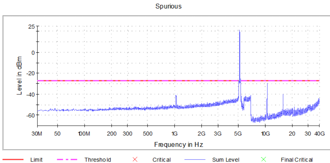
Graph 33: Antenna 1 – Spurious Emissions Channel 48 Transmitting (5240MHz) - Setting 20
