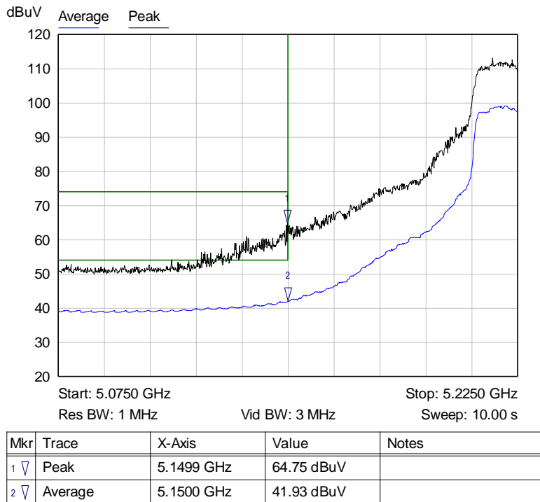
Graph 57: Antenna 1 – Channel 44 Band Edge at the Restricted Band Plot – Setting 20
