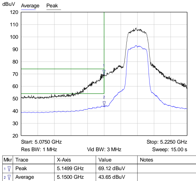
Graph 40: Antenna 0 – Channel 36 Band Edge at the Restricted Band Plot – Setting 13
