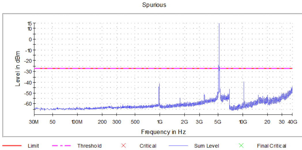
Graph 26: Antenna 0 – Spurious Emissions Channel 36 Transmitting (5180MHz) - Setting 13
