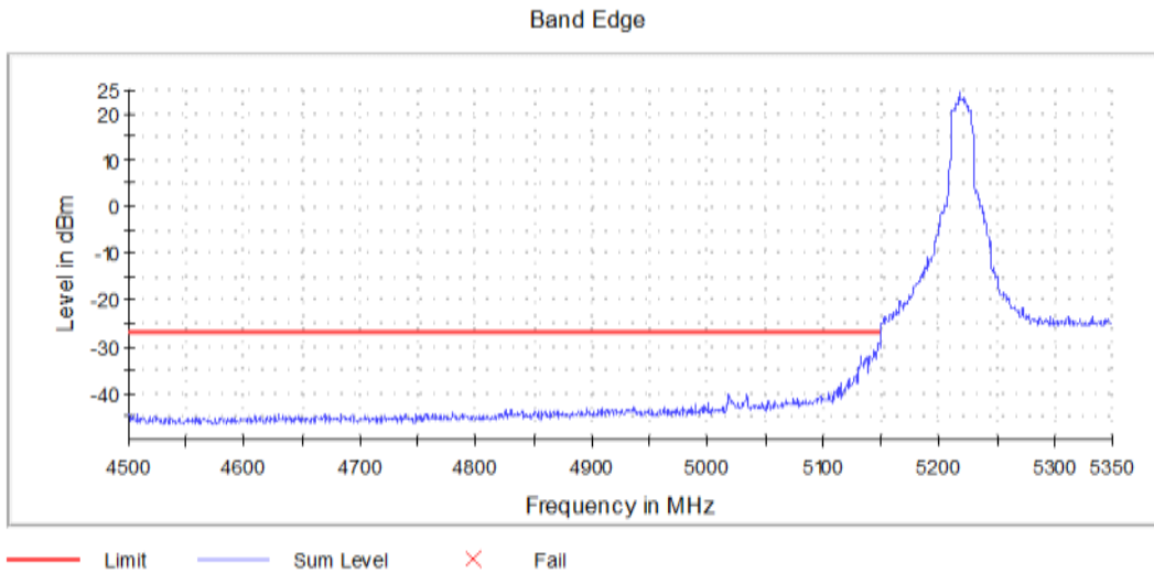
Graph 22: Antenna 1 – Lower Band Edge Channel 44 Transmitting (5220MHz) – Setting 20
