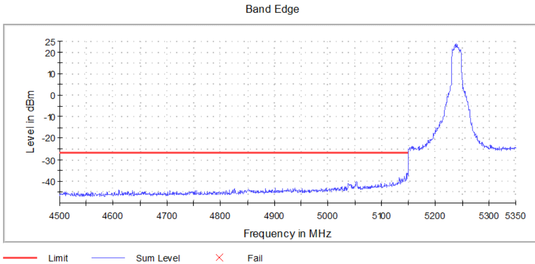
Graph 24: Antenna 1 – Lower Band Edge Channel 48 Transmitting (5240MHz) - Setting 20
