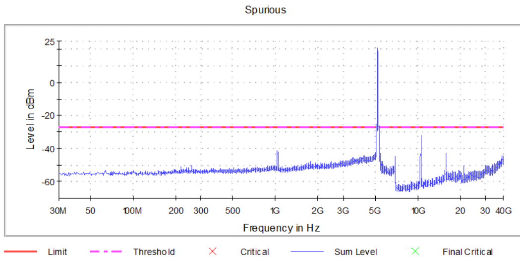
Graph 29: Antenna 0 – Spurious Emissions Channel 48 Transmitting (5240MHz) - Setting 20
