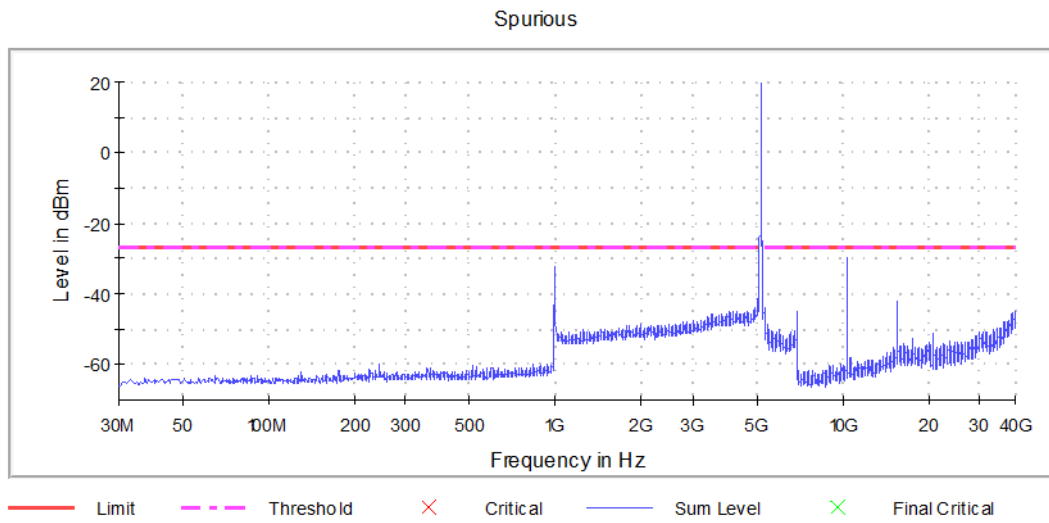
Graph 31: Antenna 1 – Spurious Emissions Channel 40 Transmitting (5200MHz) - Setting 18
