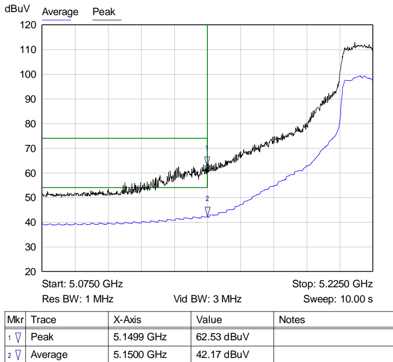
Graph 45: Antenna 1 – Channel 44 Band Edge at the Restricted Band Plot – Setting 20
