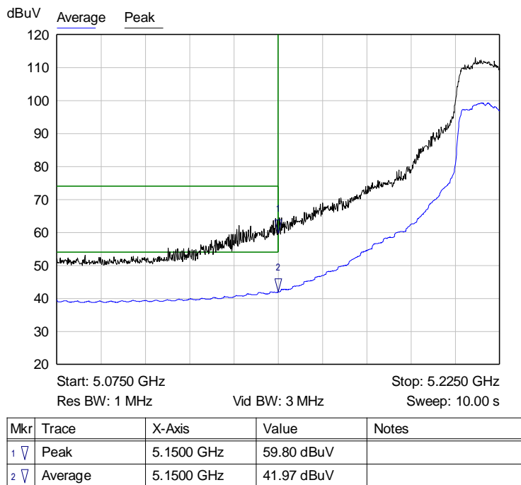
Graph 39: Antenna 1 – Channel 44 Band Edge at the Restricted Band Plot – Setting 20
