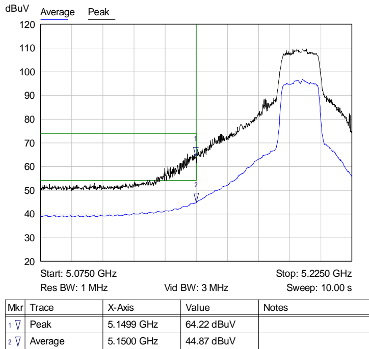
Graph 56: Antenna 1 – Channel 40 Band Edge at the Restricted Band Plot – Setting 18
