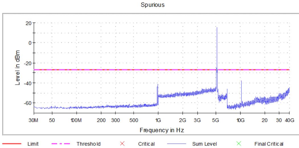
Graph 30: Antenna 1 – Spurious Emissions Channel 36 Transmitting (5180MHz) - Setting 13
