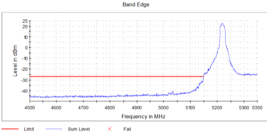
Graph 14: Antenna 0 – Lower Band Edge Channel 44 Transmitting (5220MHz) – Setting 20
