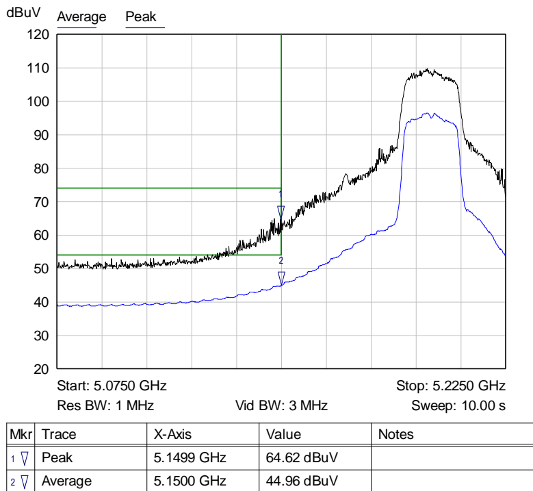
Graph 47: Antenna 0 – Channel 40 Band Edge at the Restricted Band Plot – Setting 18
