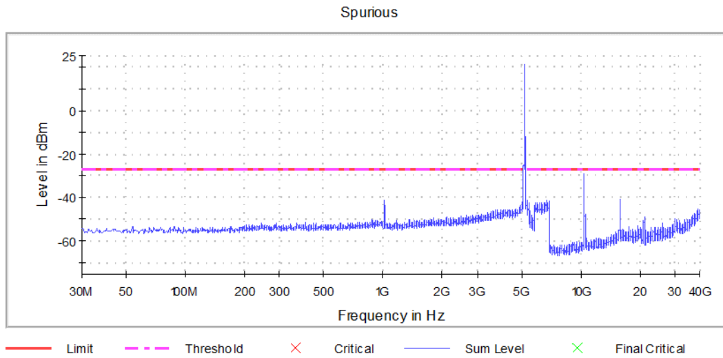
Graph 32: Antenna 1 – Spurious Emissions Channel 44 Transmitting (5220MHz) - Setting 20
