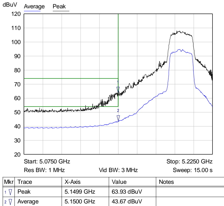
Graph 50: Antenna 1 – Channel 40 Band Edge at the Restricted Band Plot – Setting 18
