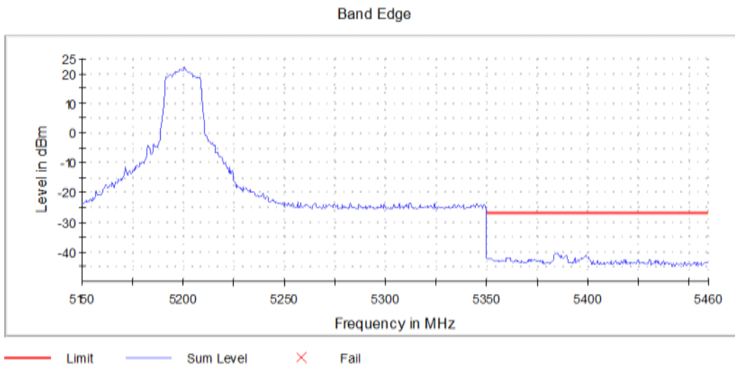
Graph 13: Antenna 0 – Upper Band Edge Channel 40 Transmitting (5200MHz) - Setting 18
