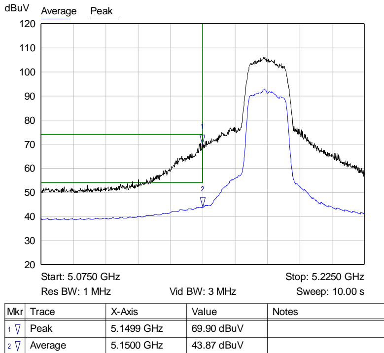
Graph 46: Antenna 0 – Channel 36 Band Edge at the Restricted Band Plot – Setting 13
