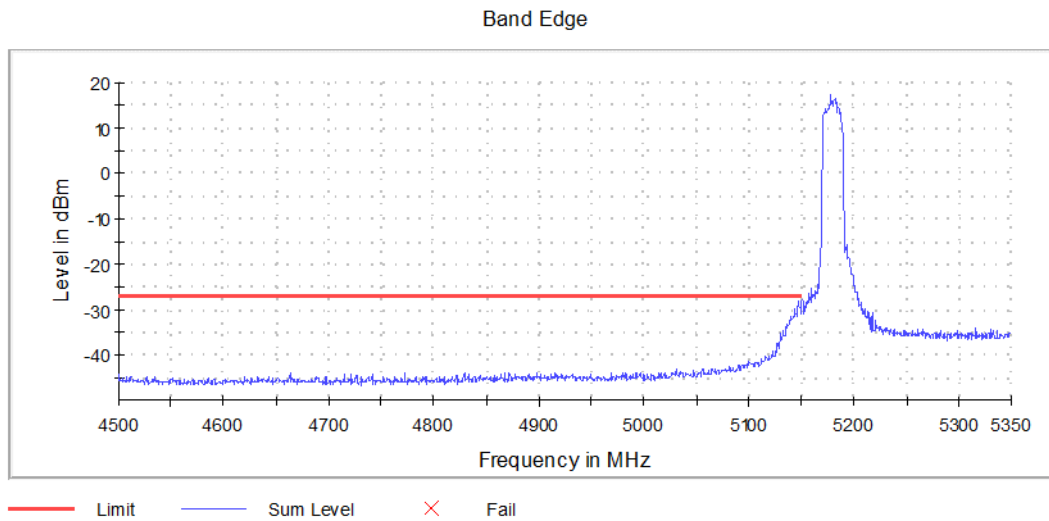
Graph 10: Antenna 0 – Lower Band Edge Channel 36 Transmitting (5180MHz) - Setting 13
