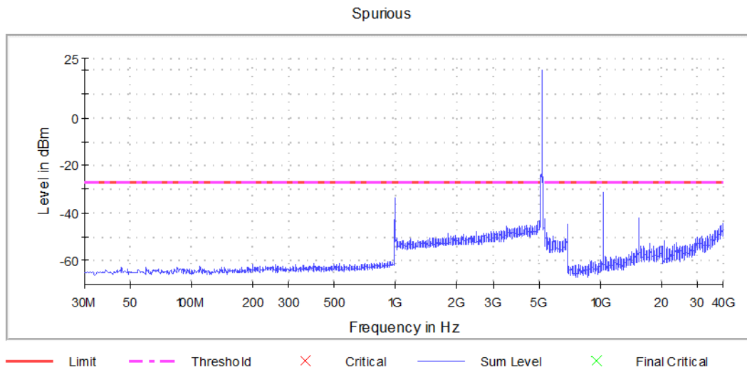
Graph 27: Antenna 0 – Spurious Emissions Channel 40 Transmitting (5200MHz) - Setting 18
