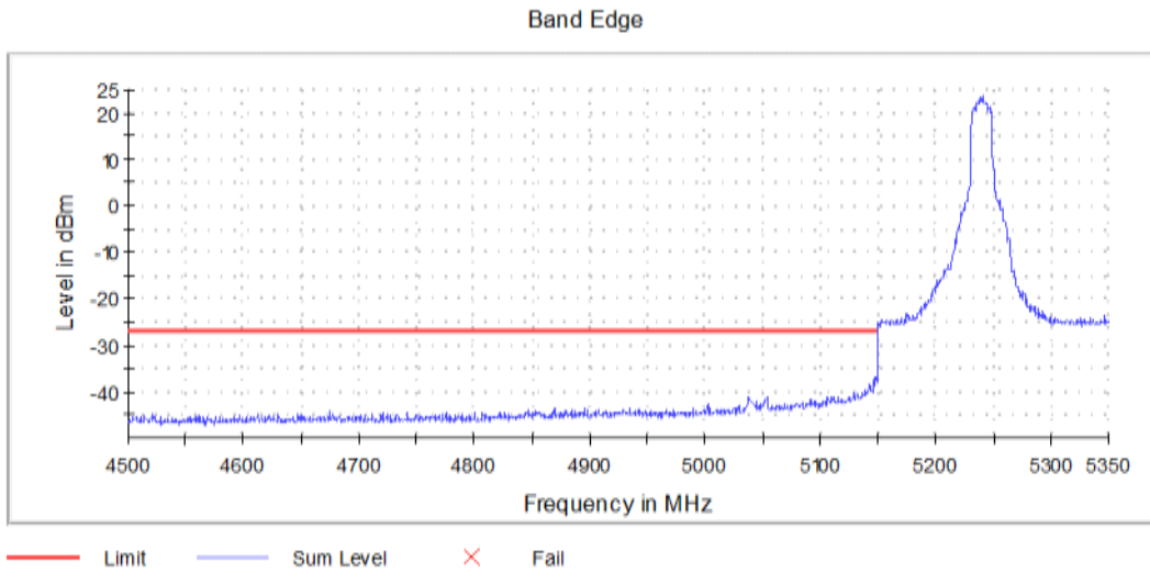
Graph 16: Antenna 0 – Lower Band Edge Channel 48 Transmitting (5240MHz) - Setting 20
