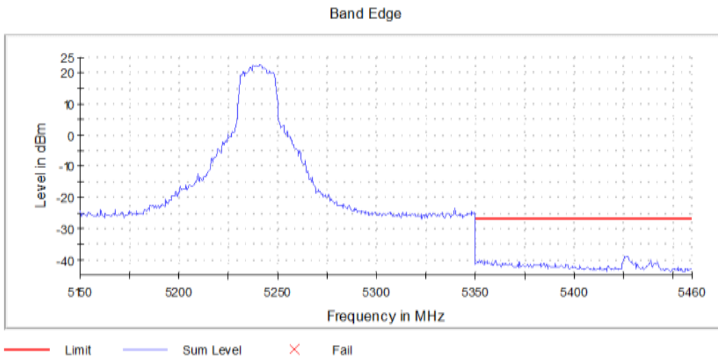
Graph 17: Antenna 0 – Upper Band Edge Channel 48 Transmitting (5240MHz) - Setting 20
