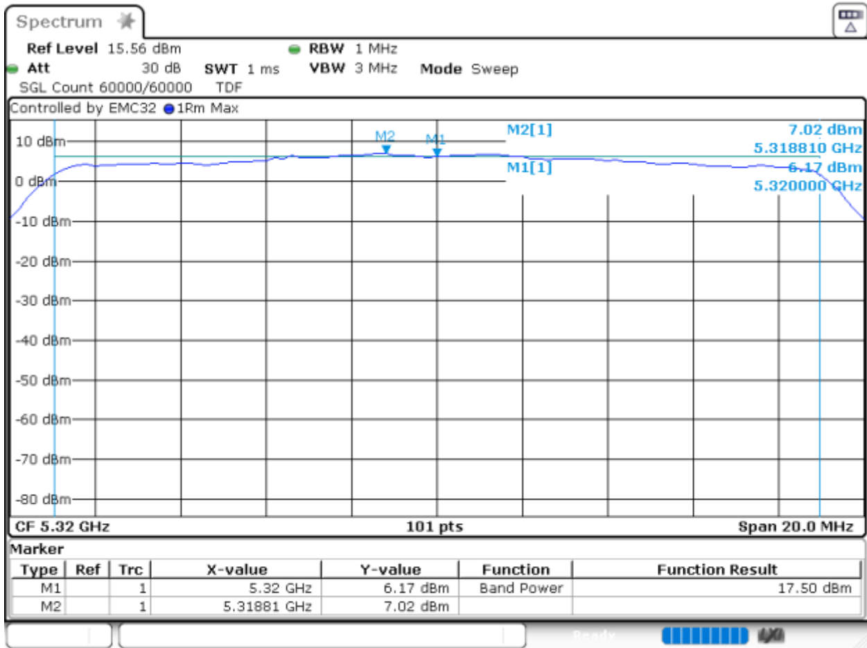
Graph 16: SA-3 Power and PSD Transmitting at 5320 MHz (Power Level 18)
