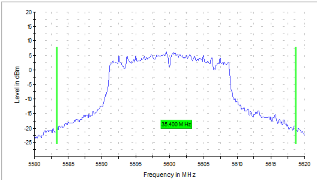
26 dB Bandwidth
