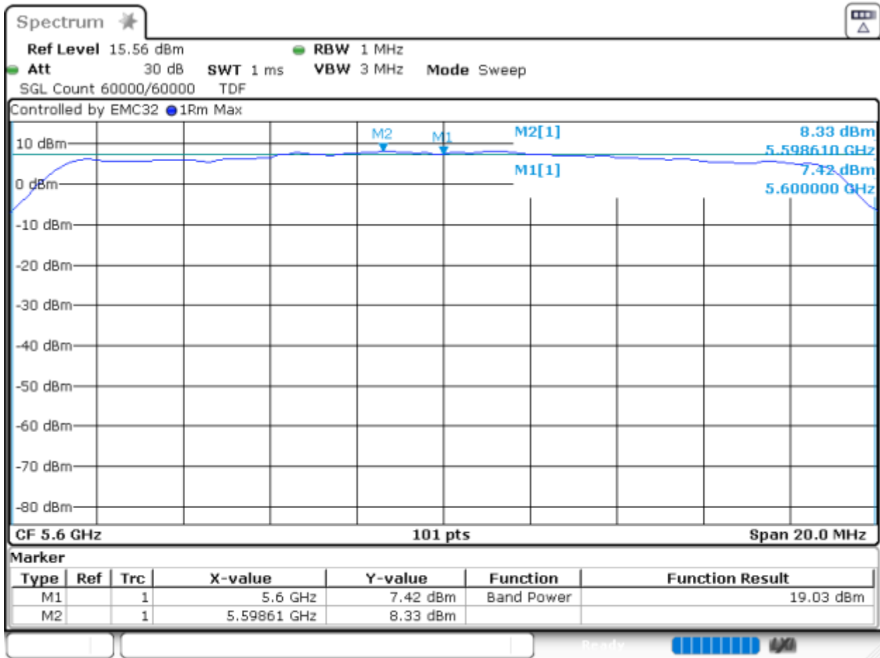
Graph 20: SA-3 Power and PSD Transmitting at 5600 MHz (Power Level 20)
