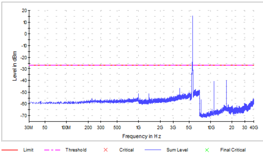
Spurious
