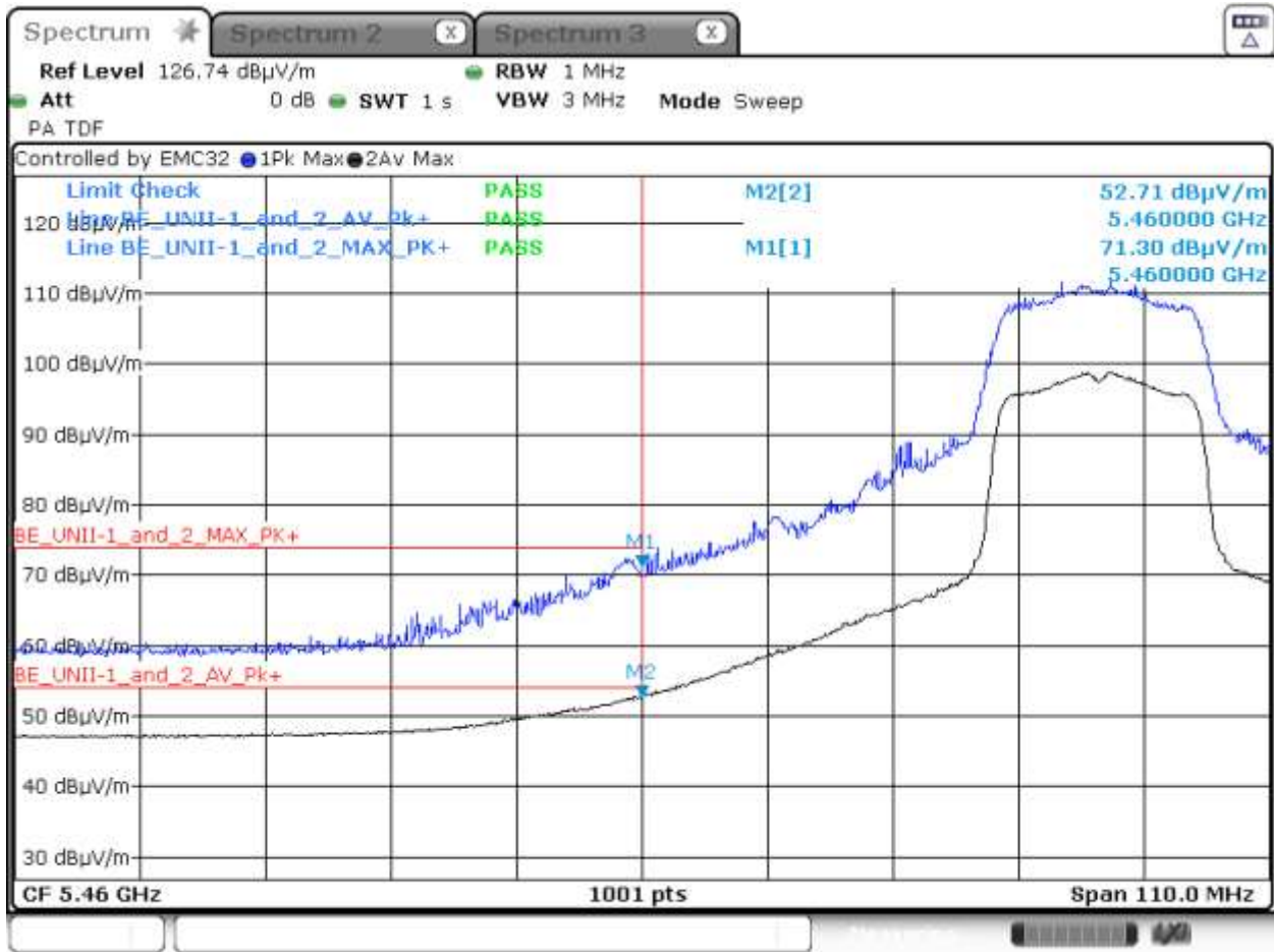
Graph 28: Radiated Restricted Band Edge Transmitting at 5520 MHz (Power Level 20, -1.3dB Margin)
