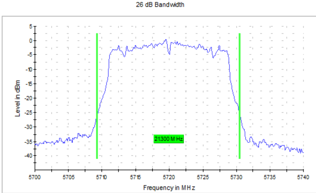
Graph 12: 26 dB Emissions Bandwidth Transmitting at 5720 MHz
