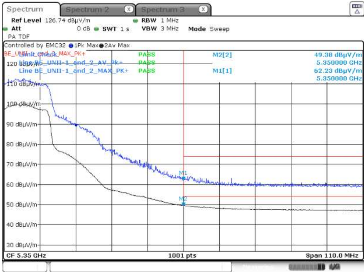
Graph 25: Radiated Restricted Band Edge Transmitting at 5300 MHz (Power Level 20, -4.6dB Margin)
