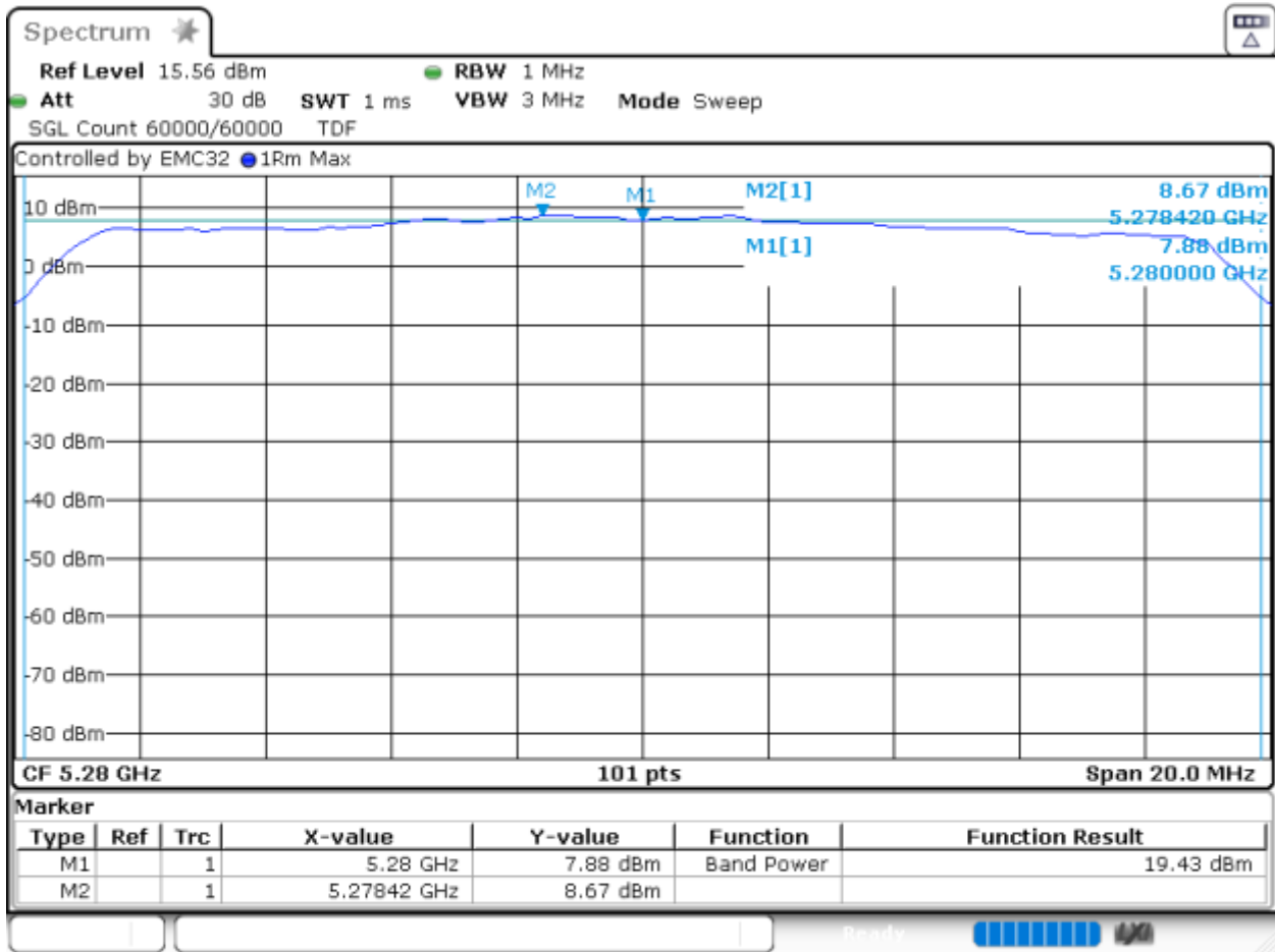
Graph 14: SA-3 Power and PSD Transmitting at 5280 MHz (Power Level 20)
