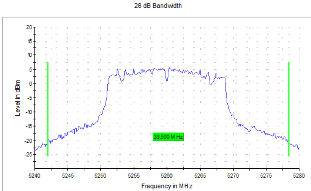
Graph 1: 26 dB Emissions Bandwidth Transmitting at 5260 MHz
