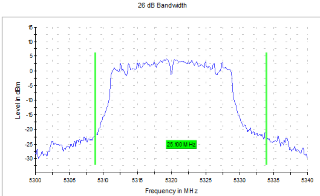
Graph 4: 26 dB Emissions Bandwidth Transmitting at 5320 MHz
