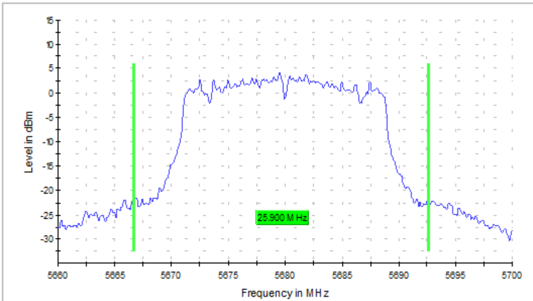
26 dB Bandwidth
