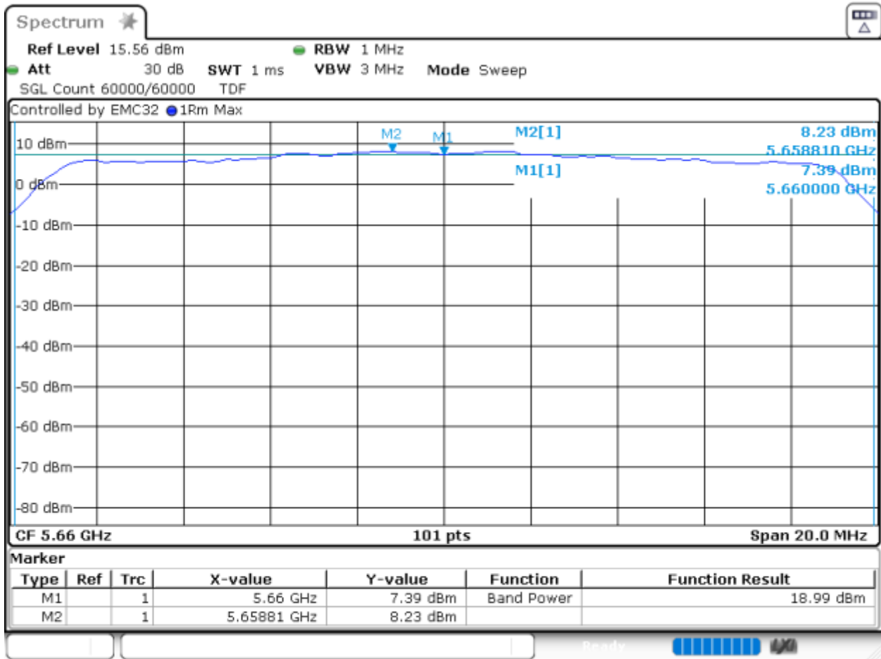
Graph 21: SA-3 Power and PSD Transmitting at 5660 MHz (Power Level 20)
