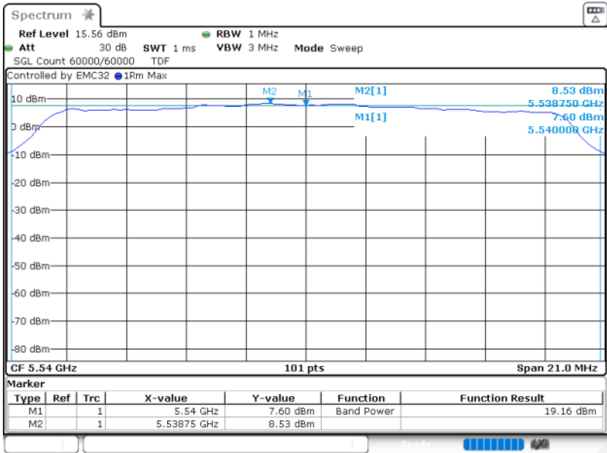
Graph 19: SA-3 Power and PSD Transmitting at 5540 MHz (Power Level 20)
