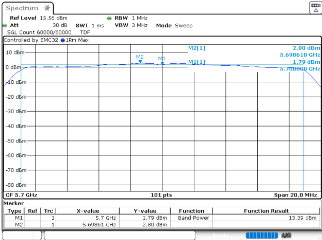
Graph 23: SA-3 Power and PSD Transmitting at 5700 MHz (Power Level 14)
