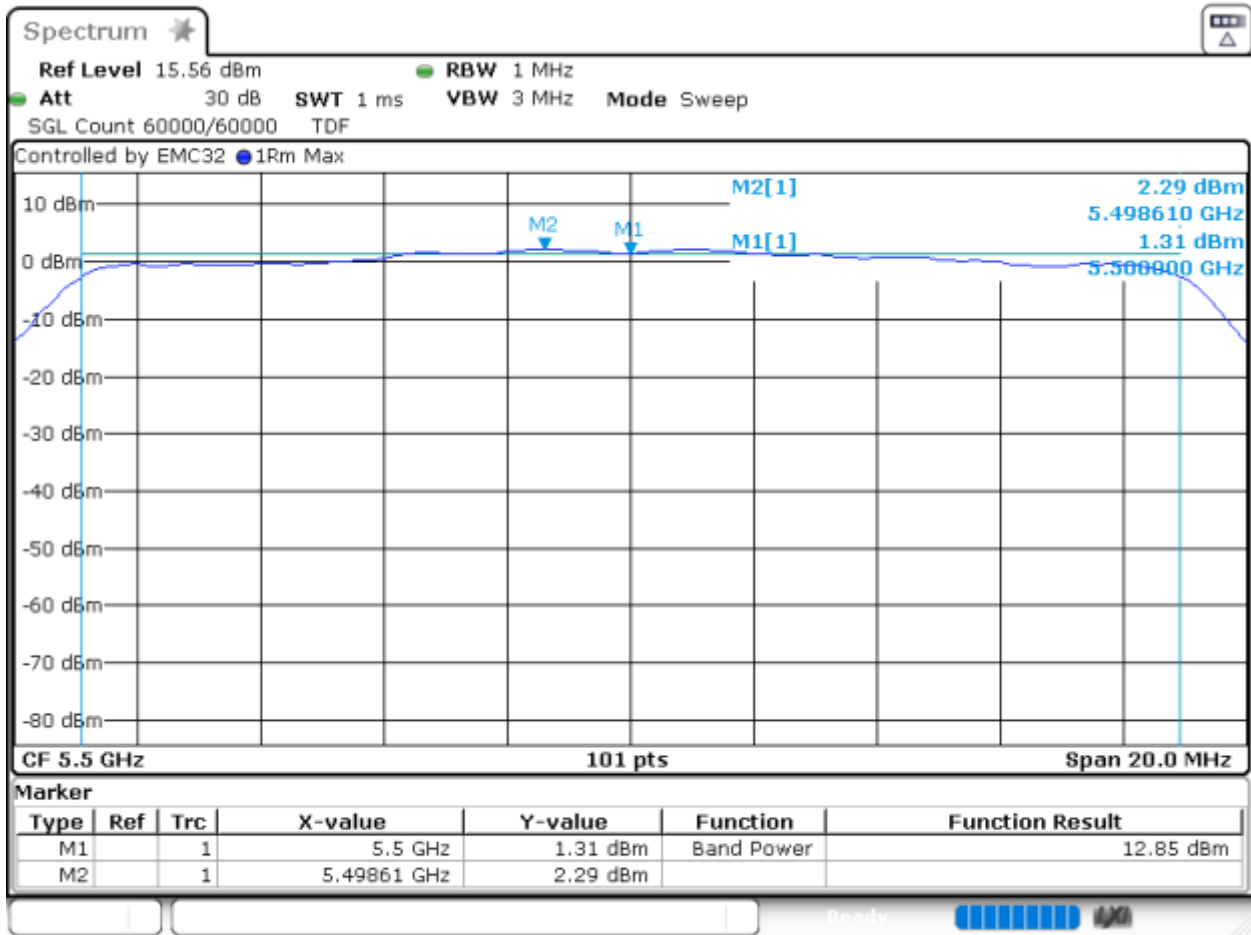
Graph 17: SA-3 Power and PSD Transmitting at 5500 MHz (Power Level 13)
