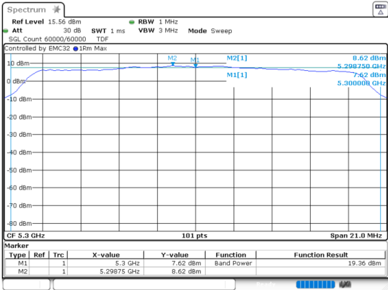
Graph 15: SA-3 Power and PSD Transmitting at 5300 MHz (Power Level 20)
