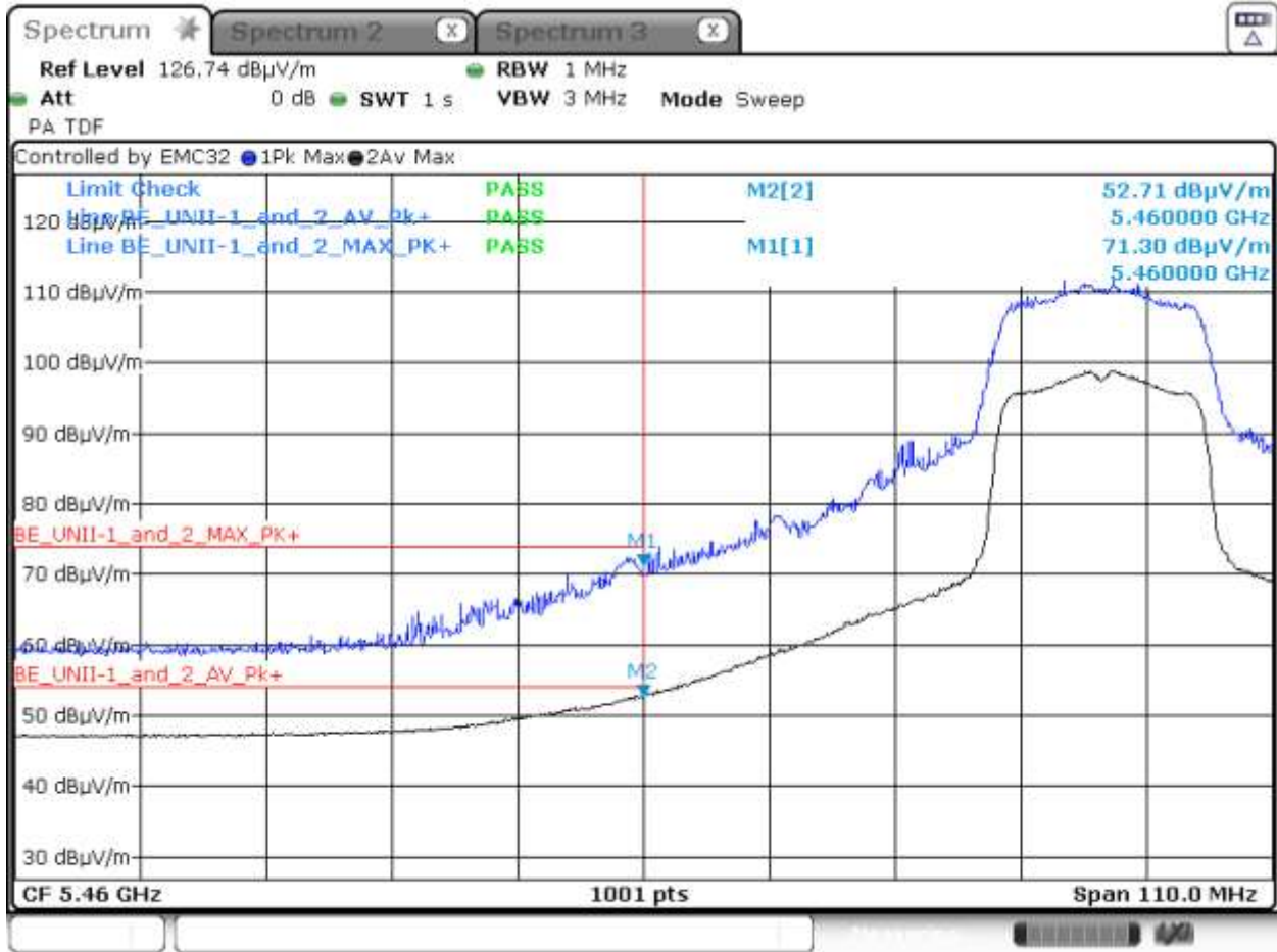
Graph 27: Radiated Restricted Band Edge Transmitting at 5500 MHz (Power Level 19, -1.3dB Margin)
