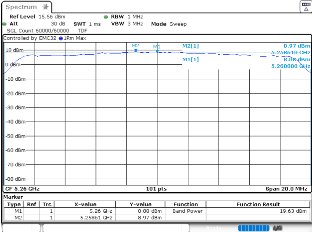
Graph 13: SA-3 Power and PSD Transmitting at 5260 MHz (Power Level 20)
