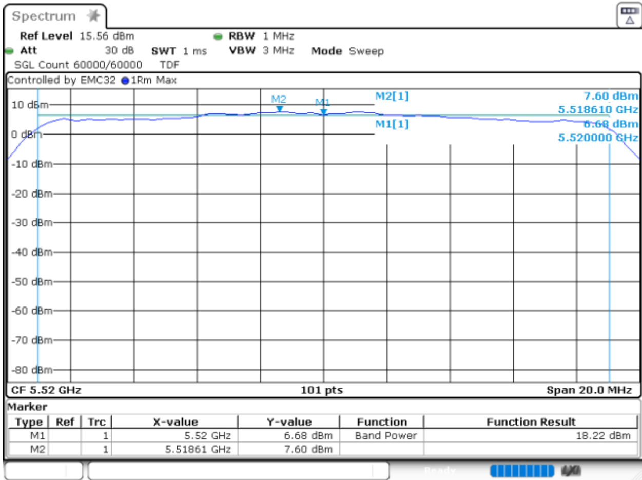
Graph 18: SA-3 Power and PSD Transmitting at 5520 MHz (Power Level 19)
