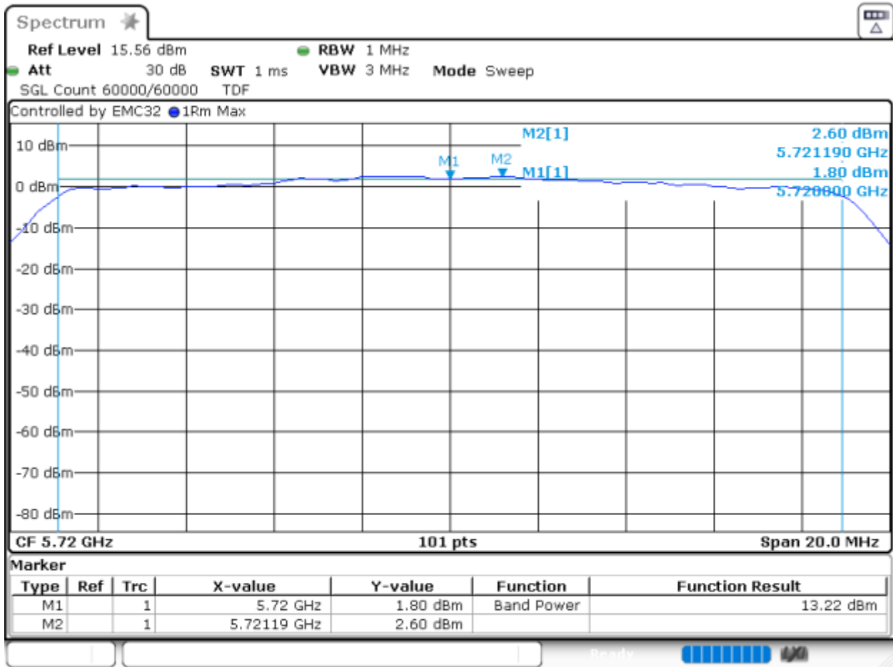
Graph 24: SA-3 Power and PSD Transmitting at 5720 MHz (Power Level 14)
