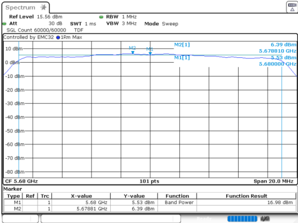
Graph 22: SA-3 Power and PSD Transmitting at 5680 MHz (Power Level 18)
