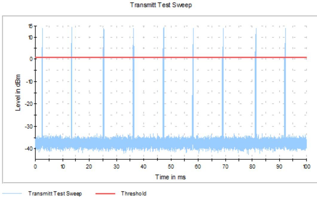
Graph 1: Normal Operation Before Radar Ping on Channel 100
