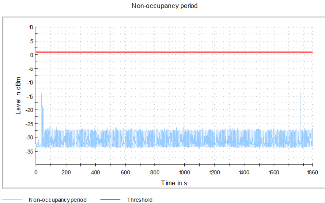
Graph 4: EUT Channel 56 Non-Occupancy Period of 30 minutes.
