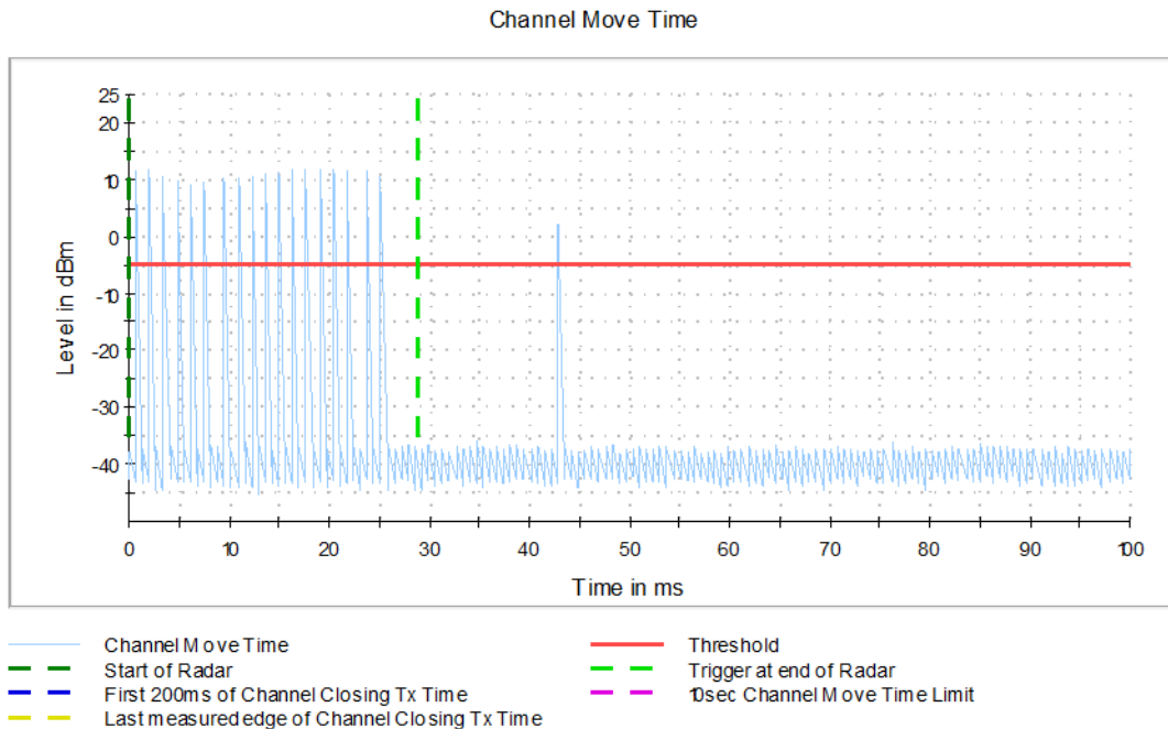
Graph 2: EUT Channel 100 Channel Close Time and Channel Move Time
