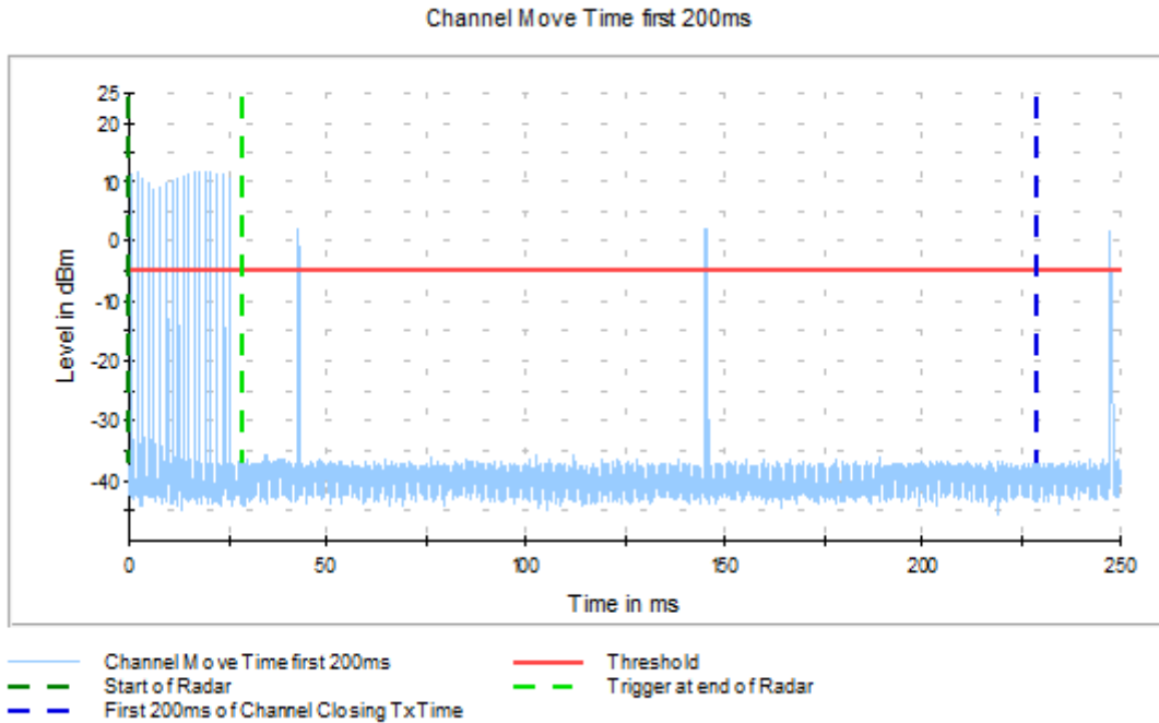
Graph 3: EUT Channel 56 First 200 ms (Channel Closing Tx Time)
