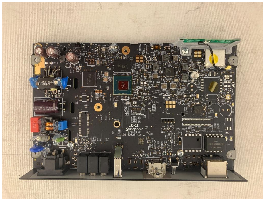
Photograph 4: Top with Heat Sink Removed
