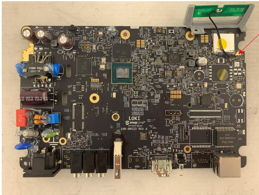
Photograph 5: Top of PCB
