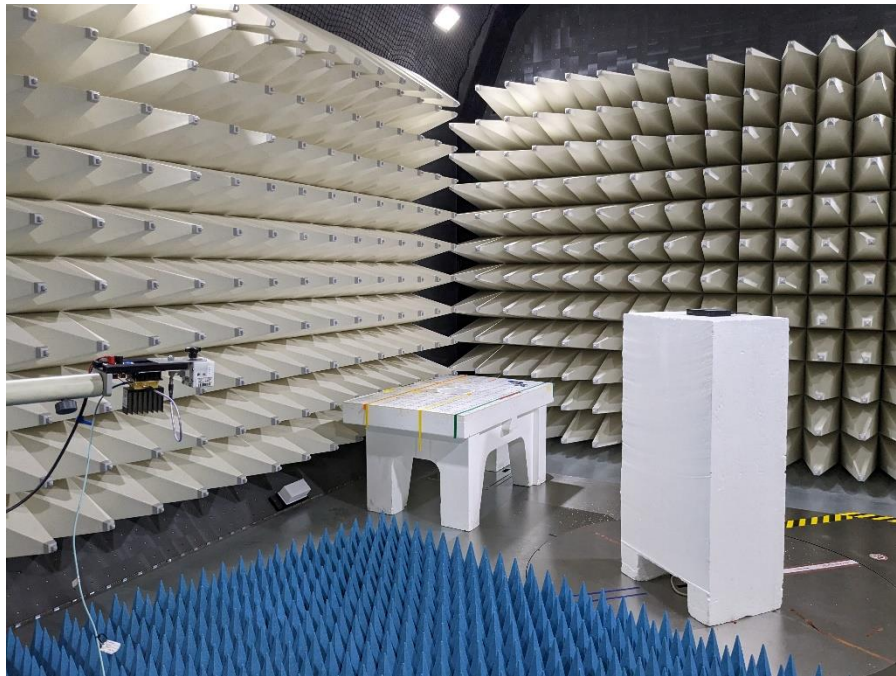
Photograph 4: Radiated Emissions 17 – 26 GHz
