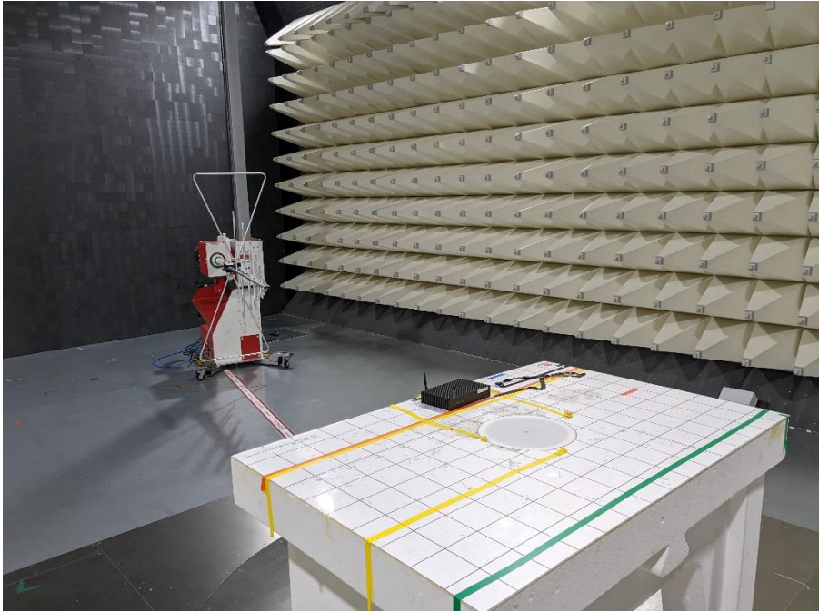
Photograph 1: Radiated Emissions 30 - 1000
