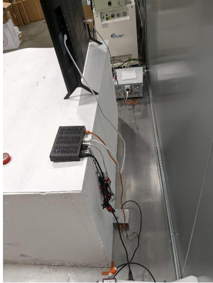
Photograph 6: Test Set Up AC Mains Conducted Emissions
