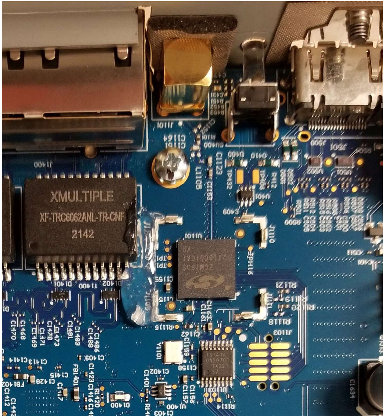
View of the Z-Wave Transceiver Circuitry with RF Shield Removed
