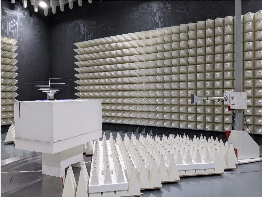
Photograph 2: Radiated Emissions 1 - 17 GHz
