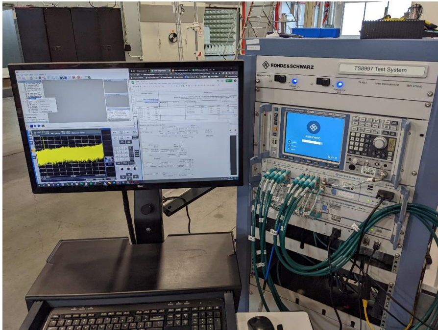
Photograph 5: Test Set Up Direct Connect
