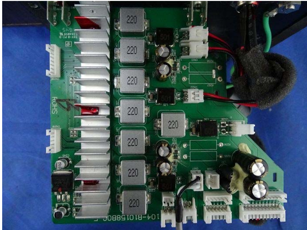
(27) EUT Photo
