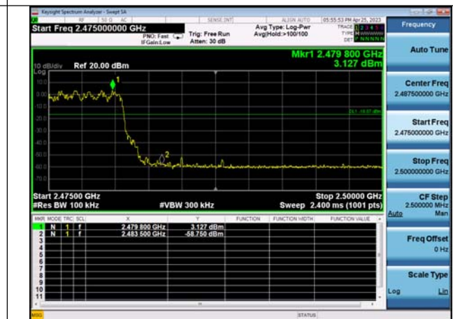
8DPSK Hopping Band edge-Right side
