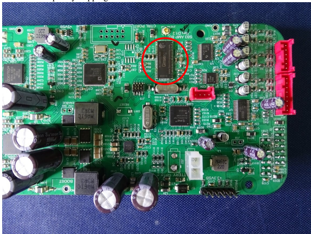
(24) EUT Photo-Frequency hopping of 2.4GHz Module
