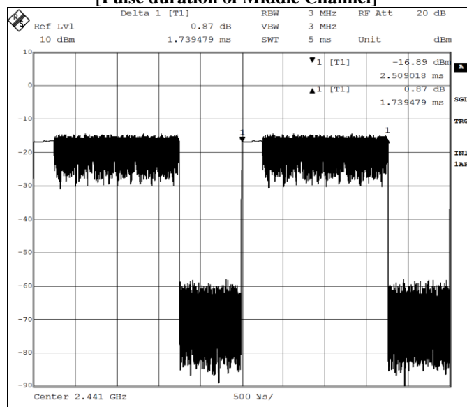
Fig. E [Pulse duration of Middle Channel]
