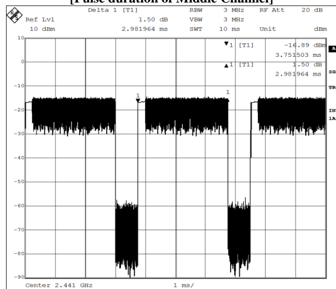
Fig. B [Pulse duration of Middle Channel]
