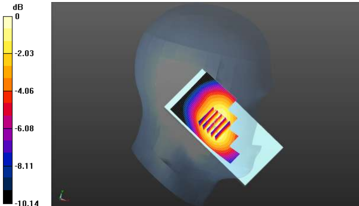
0 dB = 0.479 W/kg = -3.20 dBW/kg
