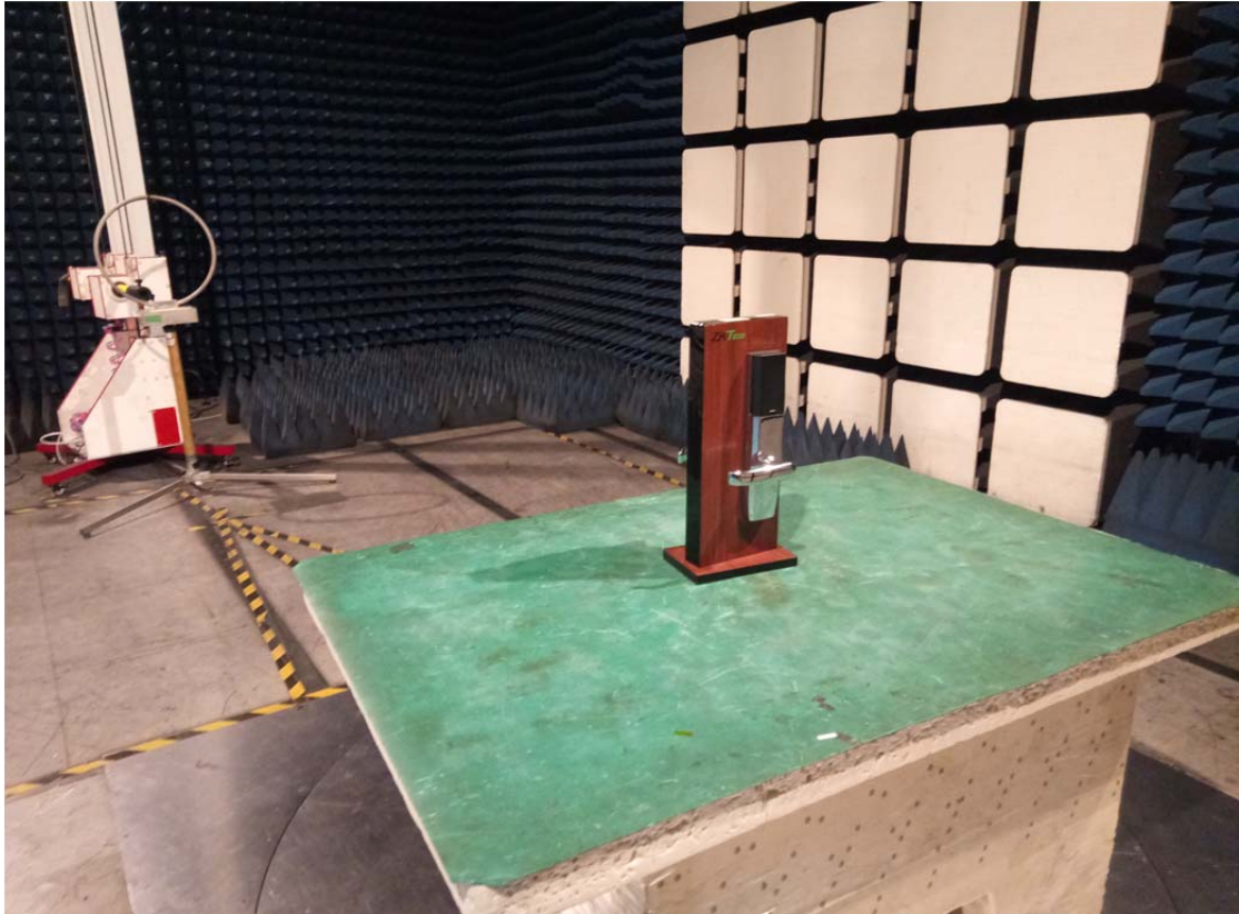
Test setup
