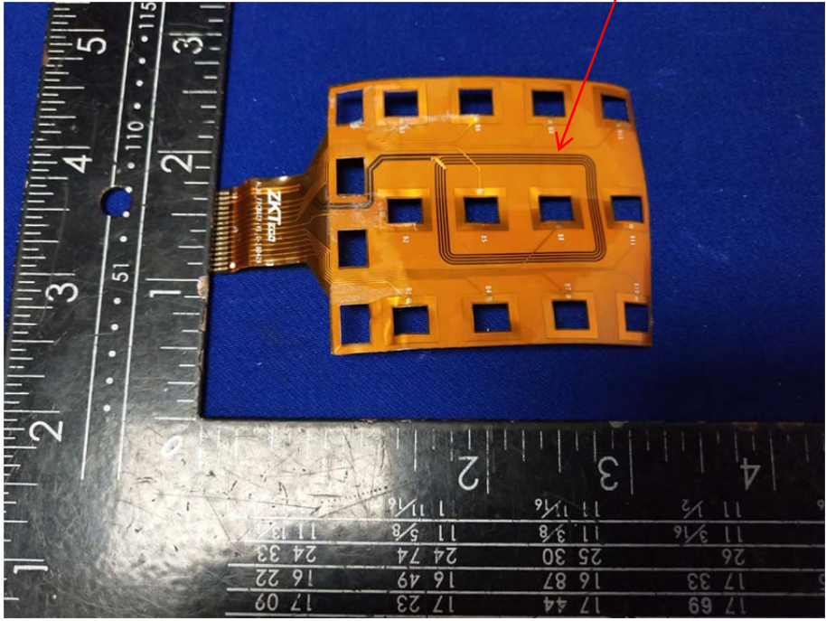
13.56MHz Antenna
