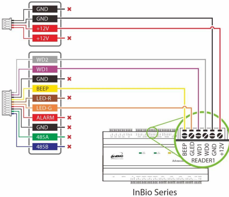
Figure 1-3 InBio Wiring
