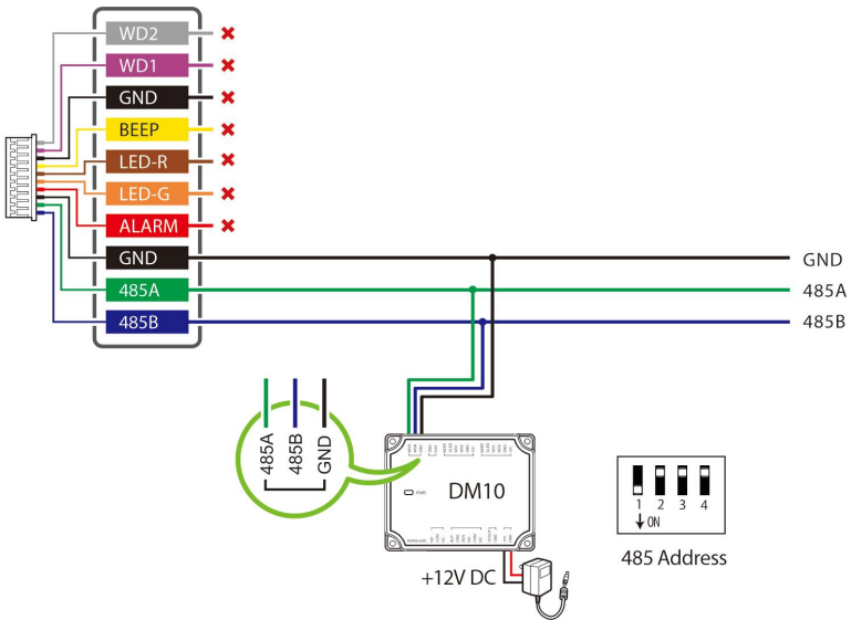
Figure 1-4 DM10 Wiring
