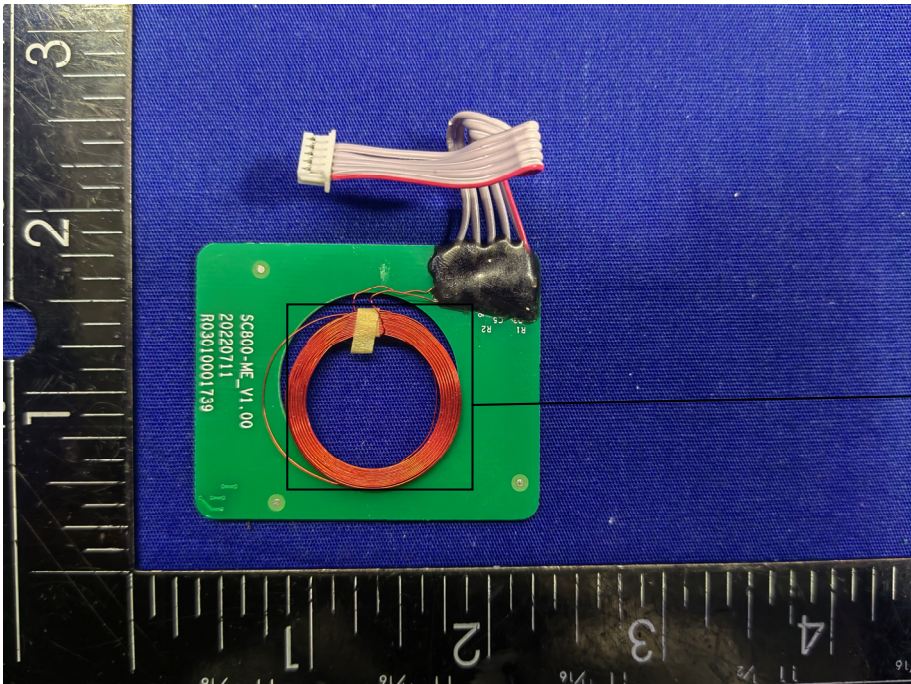
125KHz antenna
