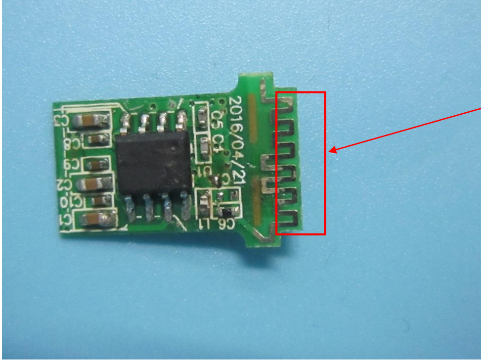
RF Antenna
