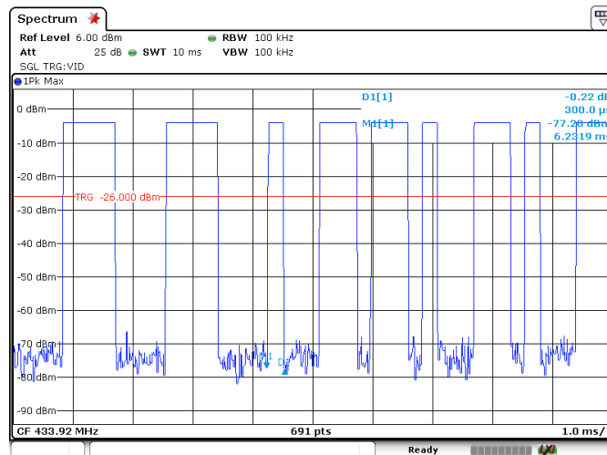
Pulse 2 width
