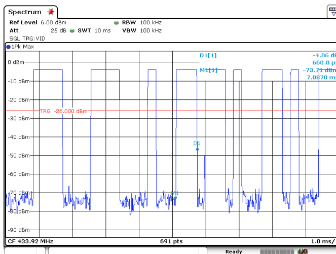
Pulse 3 width
