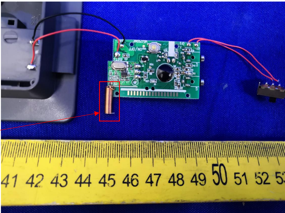
Transmitter Antenna
