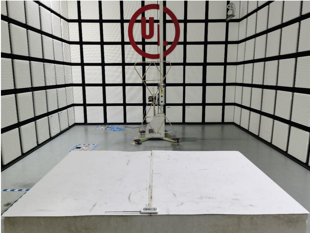
Radiated Disturbance Setup Below 30 MHz
