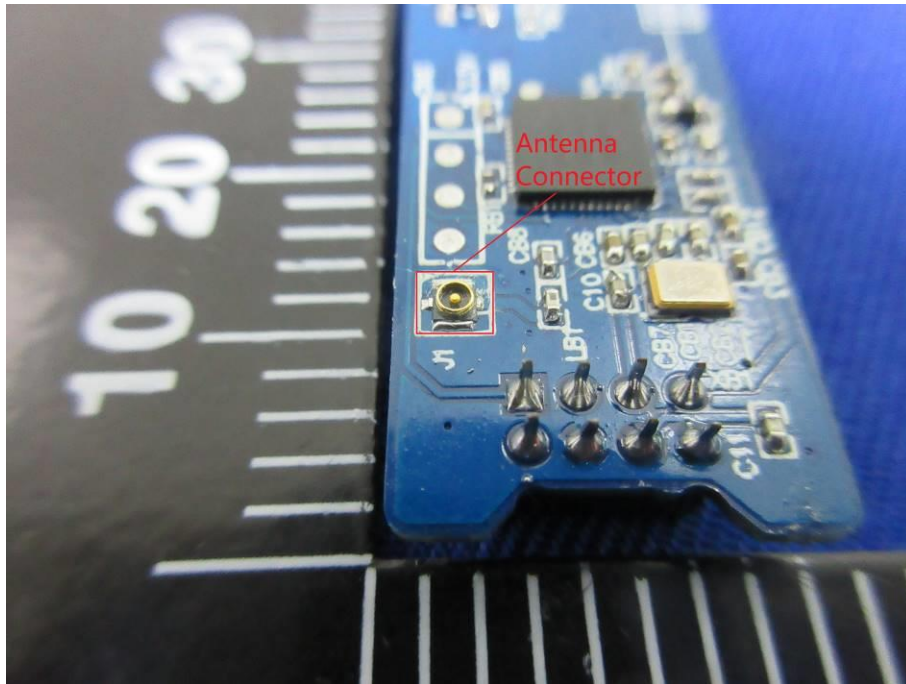
Antenna Connector-1
