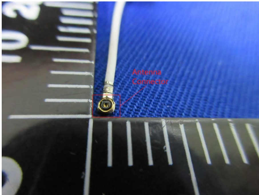
Antenna Connector-2
