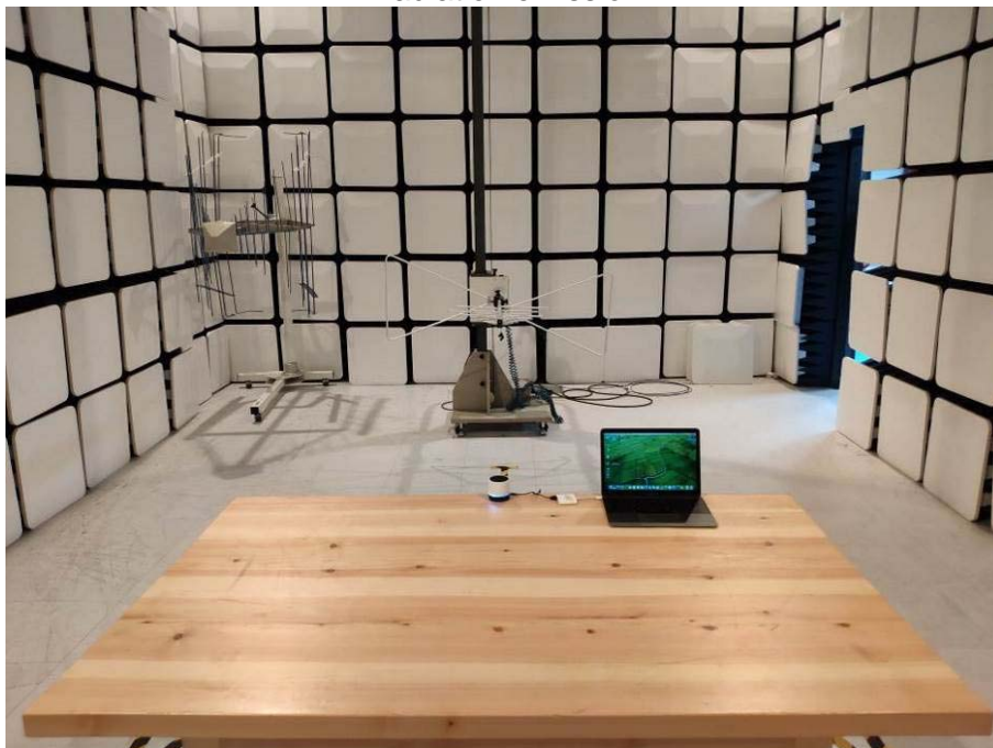
Radiation emission
