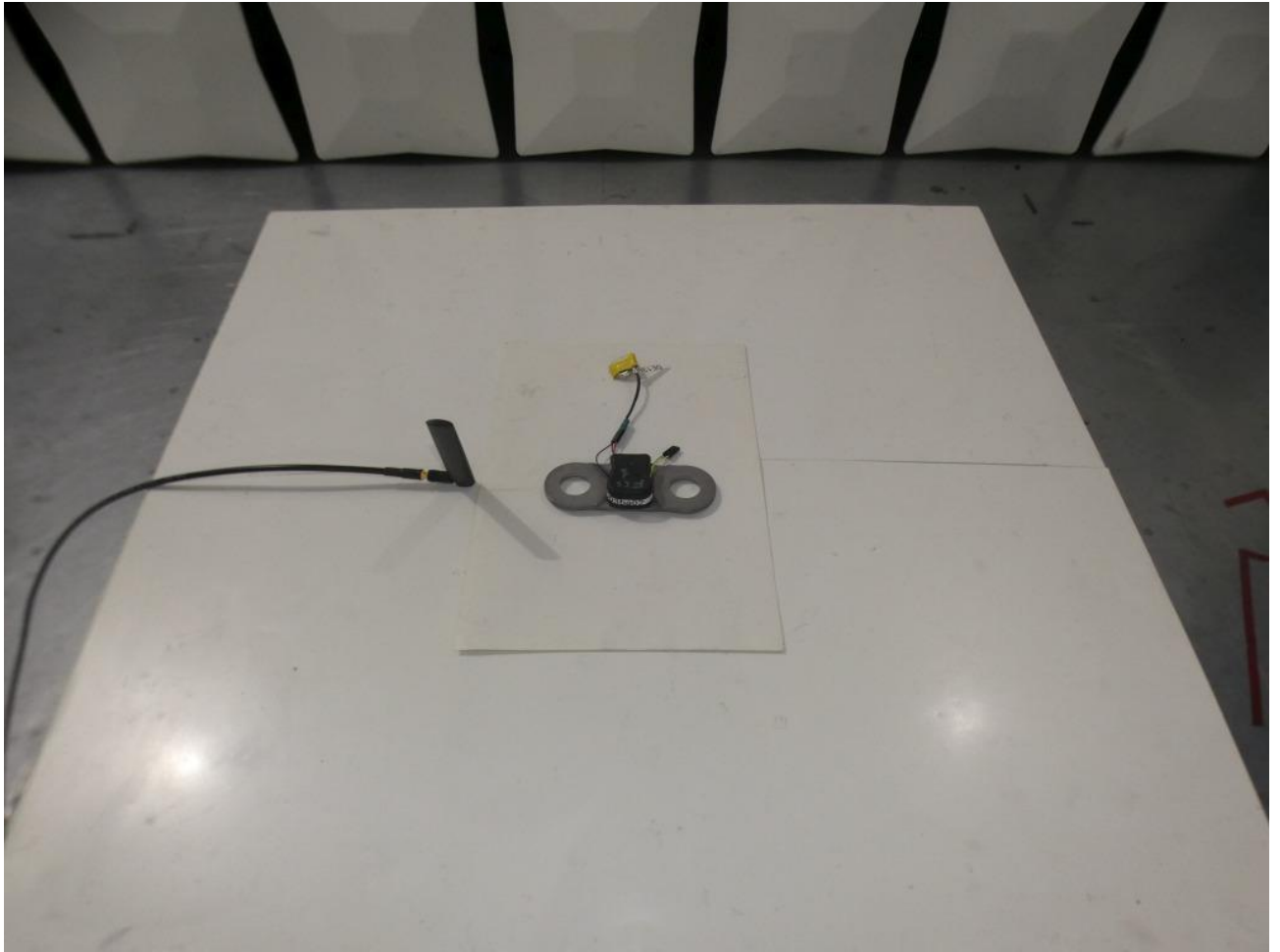
Photo 3: Test setup for radiated measurements (stand alone setup, 30 MHz - 1 GHz; FCC 15c247, detailed view)
