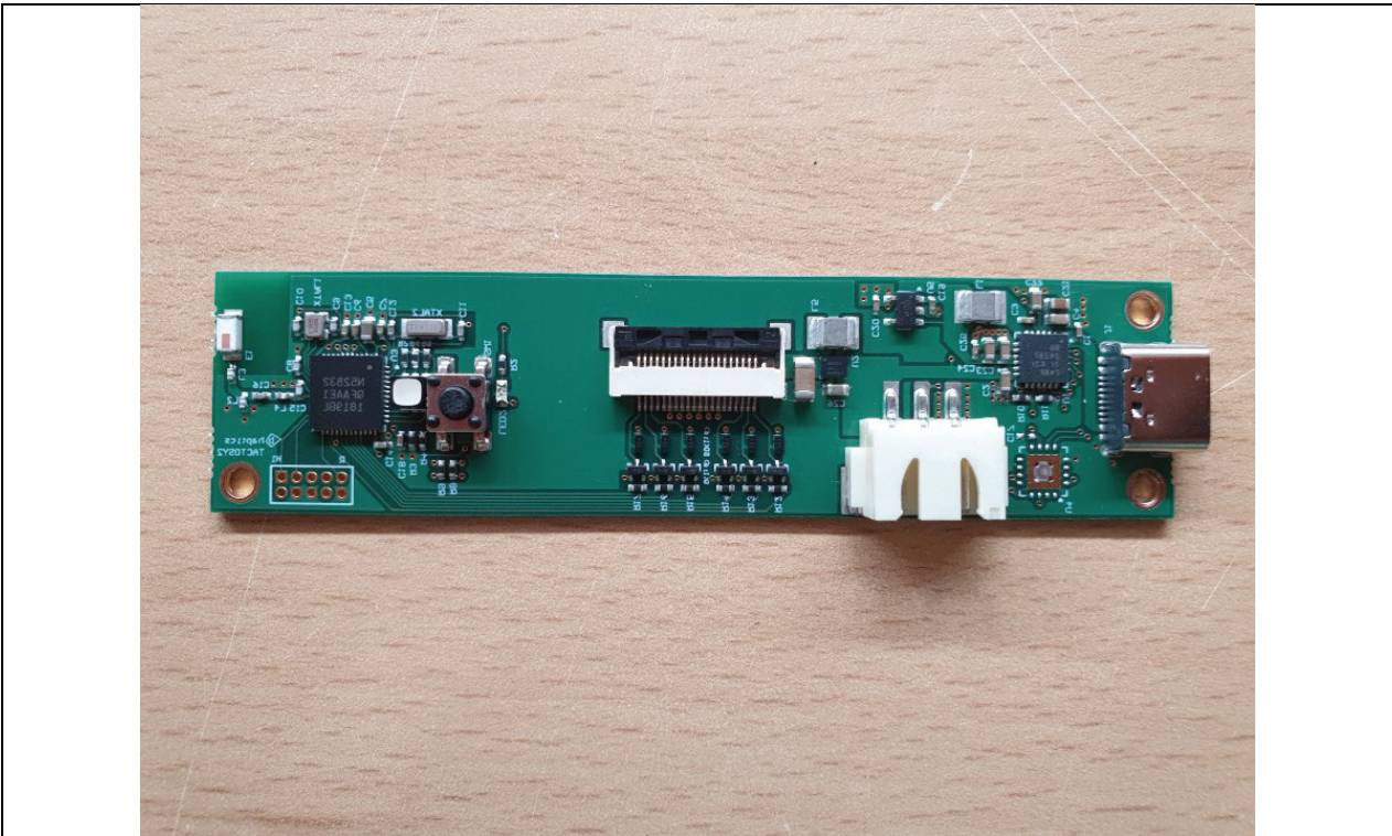
Mainboard 1
