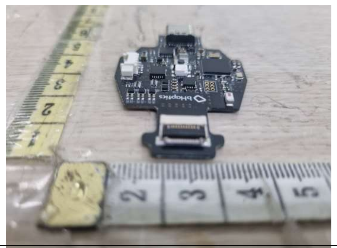
Main Board Side4
