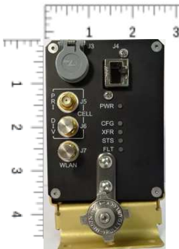
Figure 3: Front View
