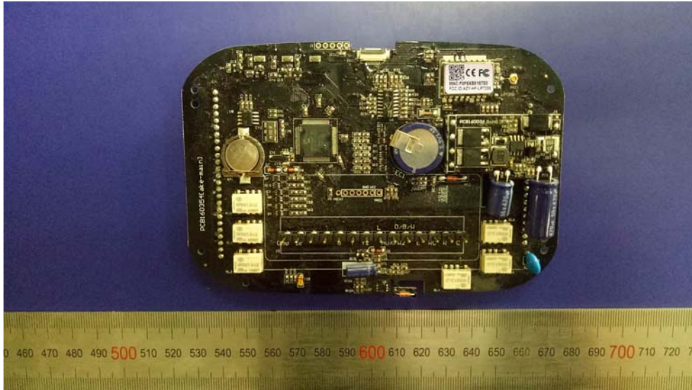
EUT – Mainboard Bottom View
