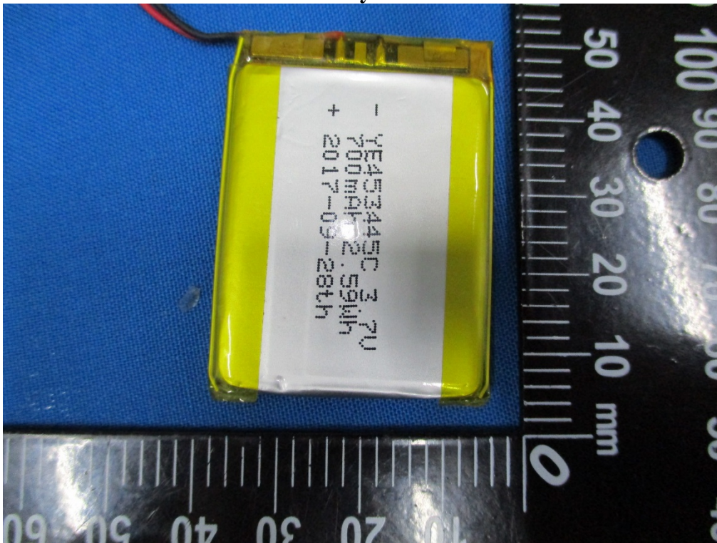
Battery View
