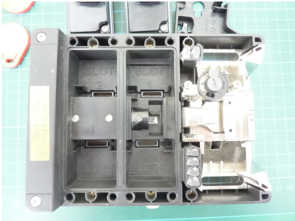
Internal view CKS2 02
