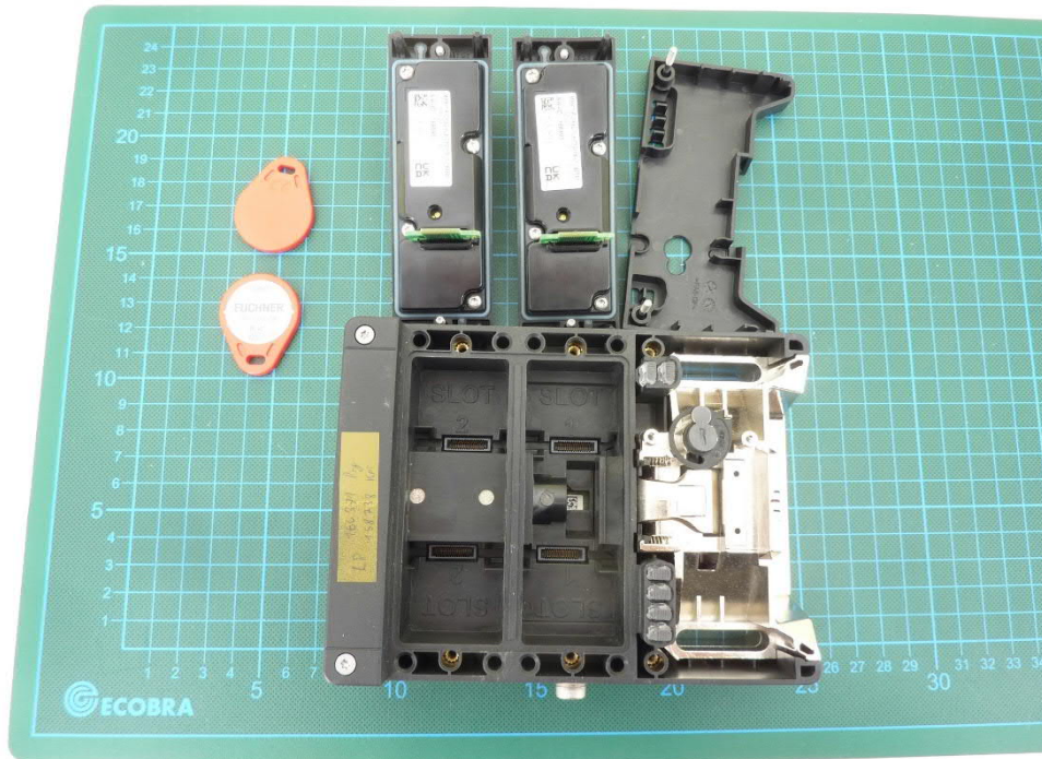
Internal view CKS2 01
