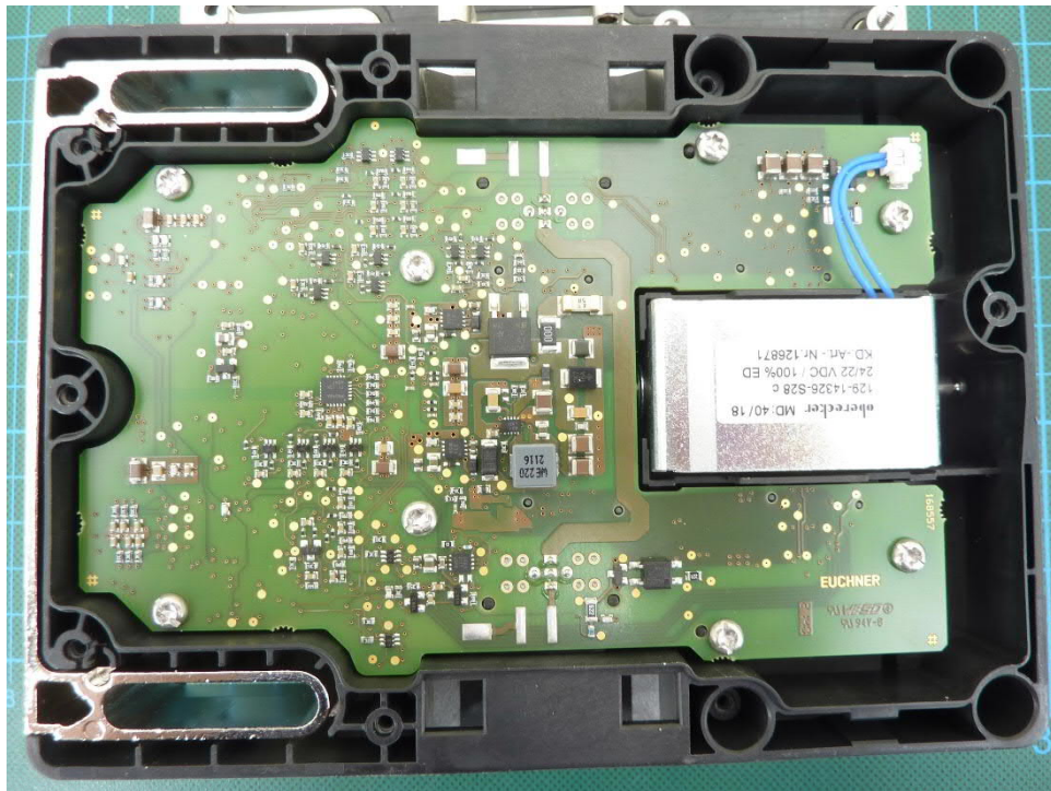
Internal view CKS2 07
