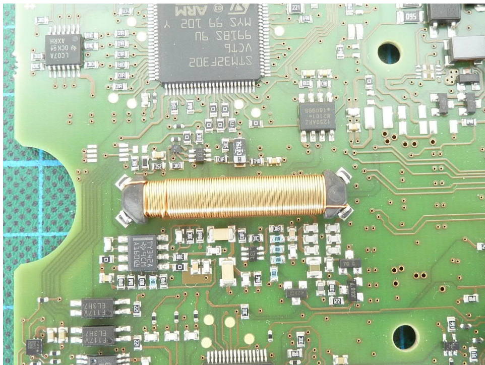
PCB view CKS2 03
