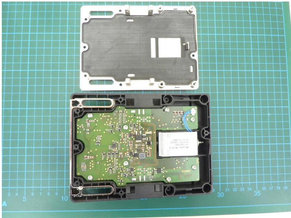
Internal view CKS2 06
