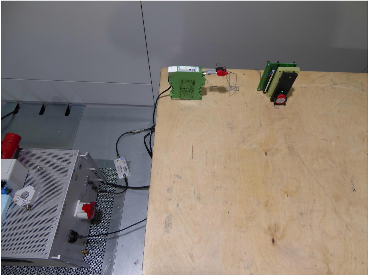
AC Mains conducted emissions test setup
