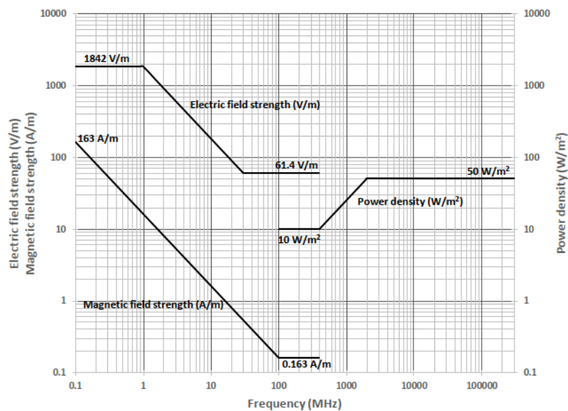
Figure 4—Graphical representations of the ERLs in Table 8 for electric and magnetic fields and plane-wave-equivalent power density—Persons permitted in restricted environments
