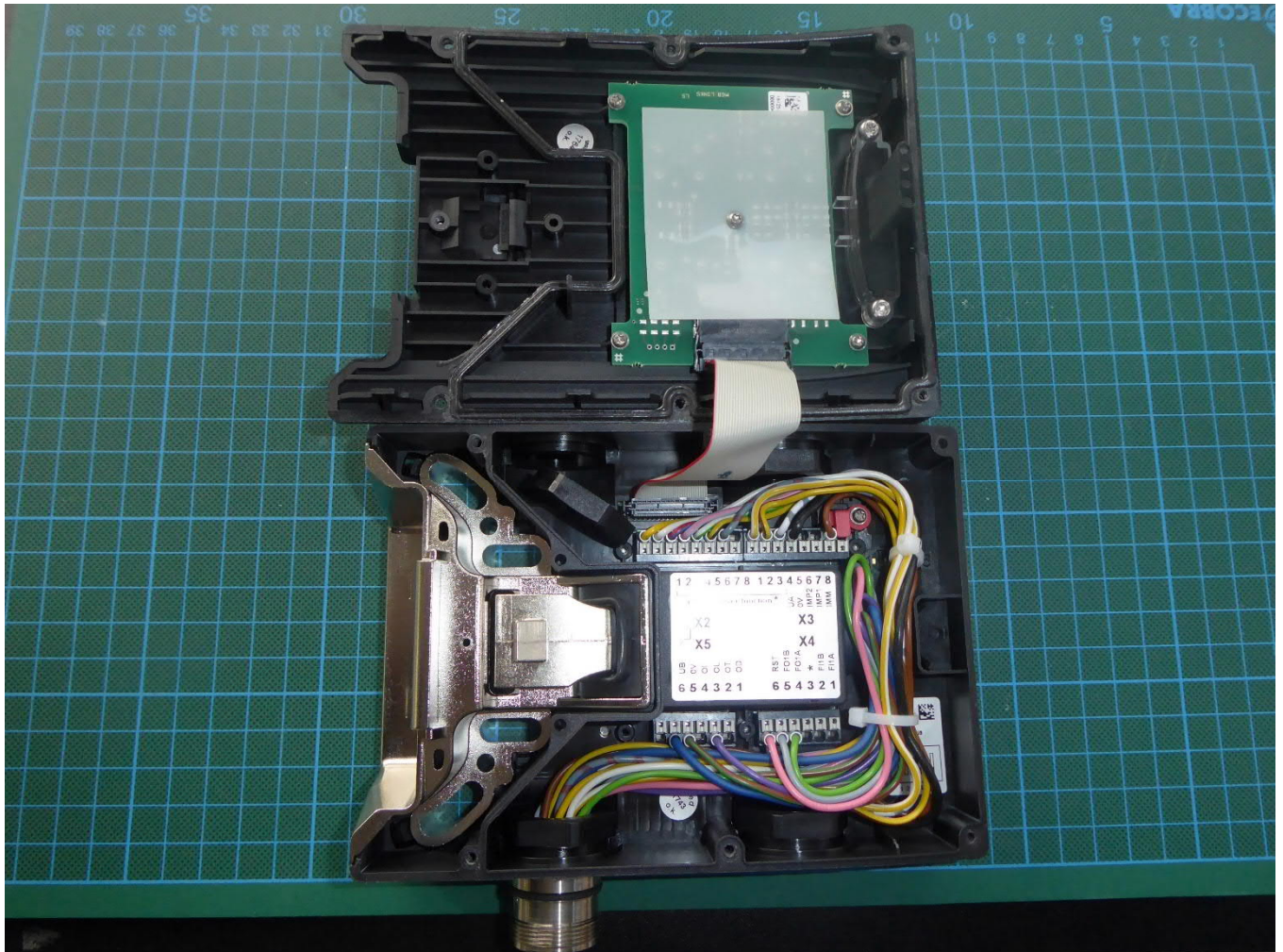
EUT, front cover removed
