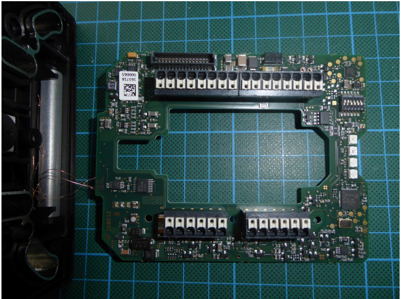
PCB, detail view (front)
