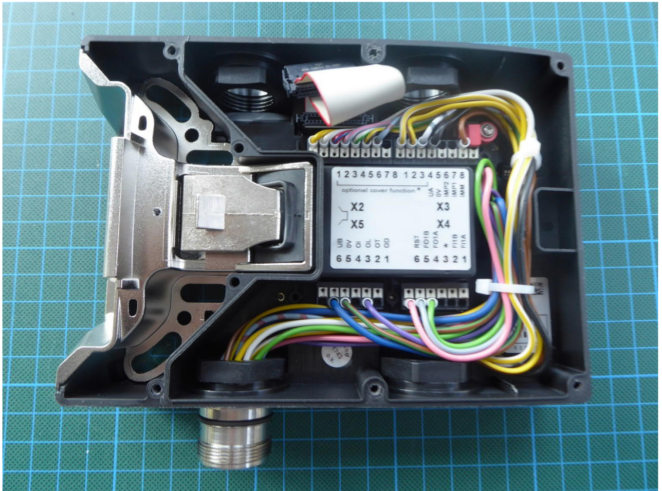
EUT, front cover removed, detail view
