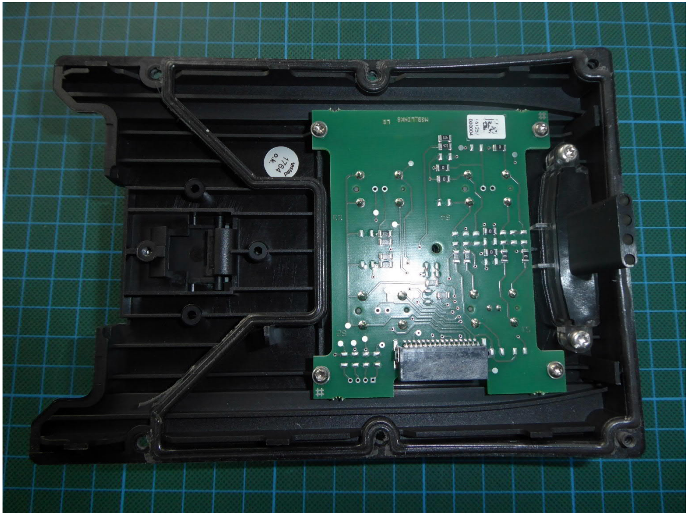
Front cover, detail view, protection removed
