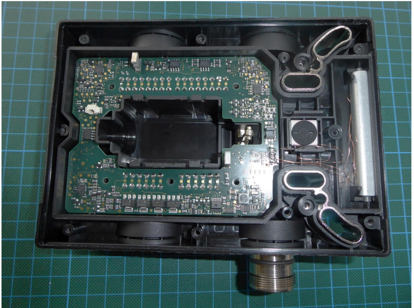
EUT, back cover removed, detail view
