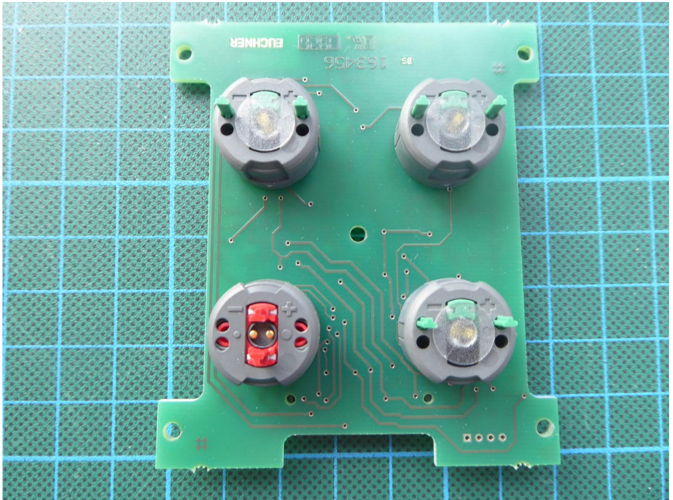
Front cover PCB, detail view (front)
