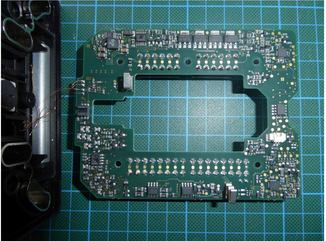
PCB, detail view (back)
