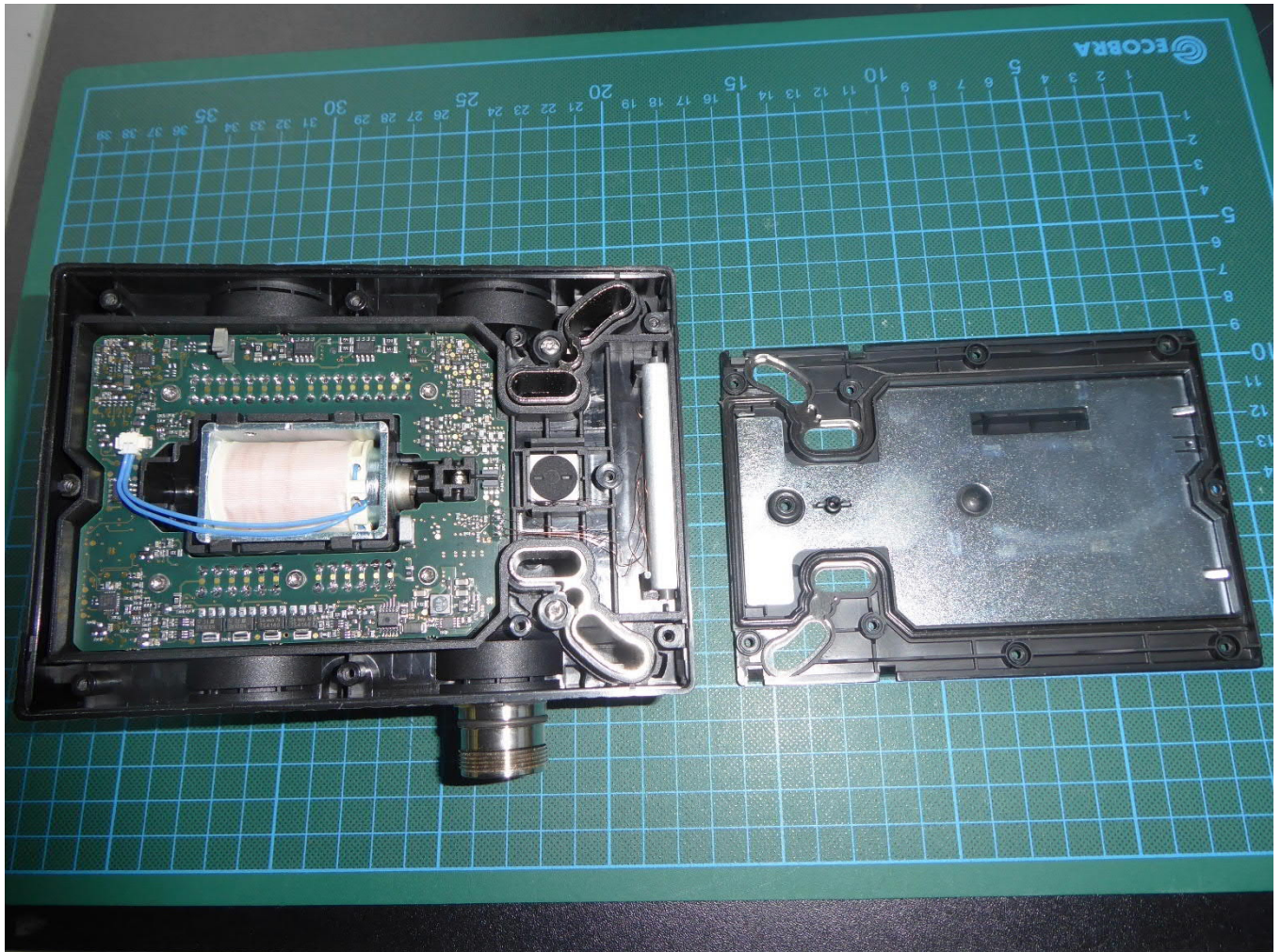
EUT, back cover removed
