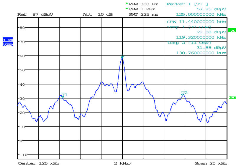
Plot 2: 99 % emission bandwidth (EUT B)
