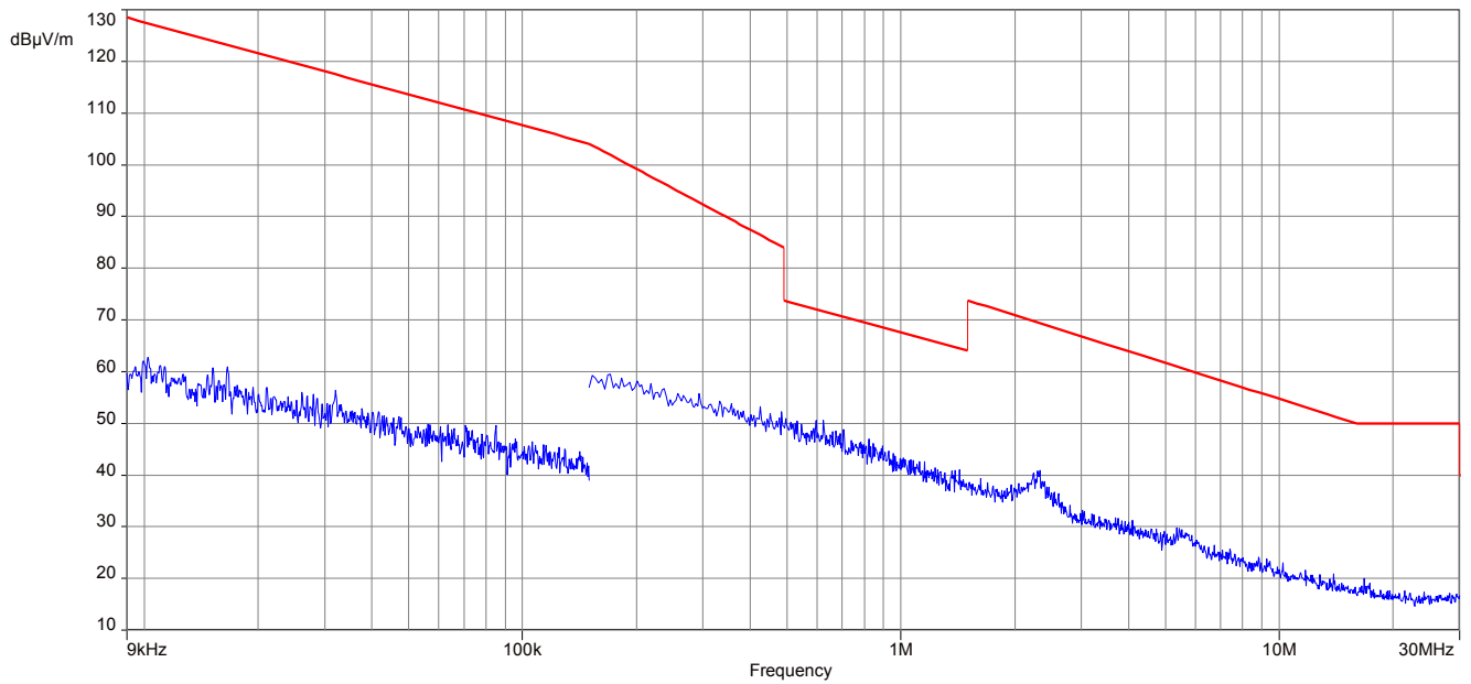
Plot 1: 9 kHz – 30 MHz, magnetic emissions EKS-A-IEXA-G01-ST02/03/04
