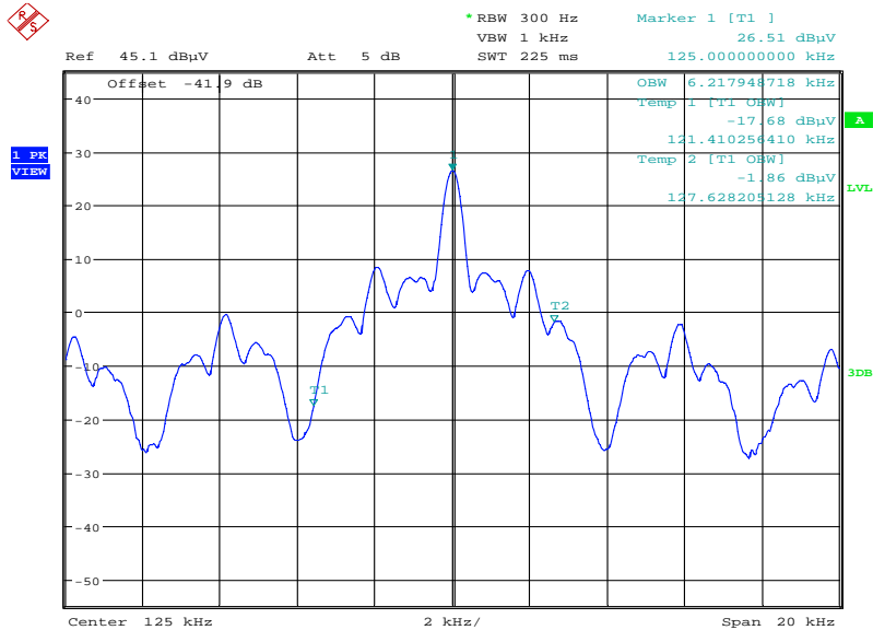
Plot 2: 99 % emission bandwidth EKS-A-IEXA-G01-ST02/03/04
