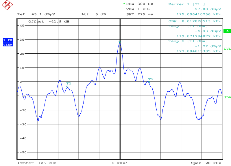
Plot 1: 99 % emission bandwidth EKS-A-IEX-G01-ST02/03
