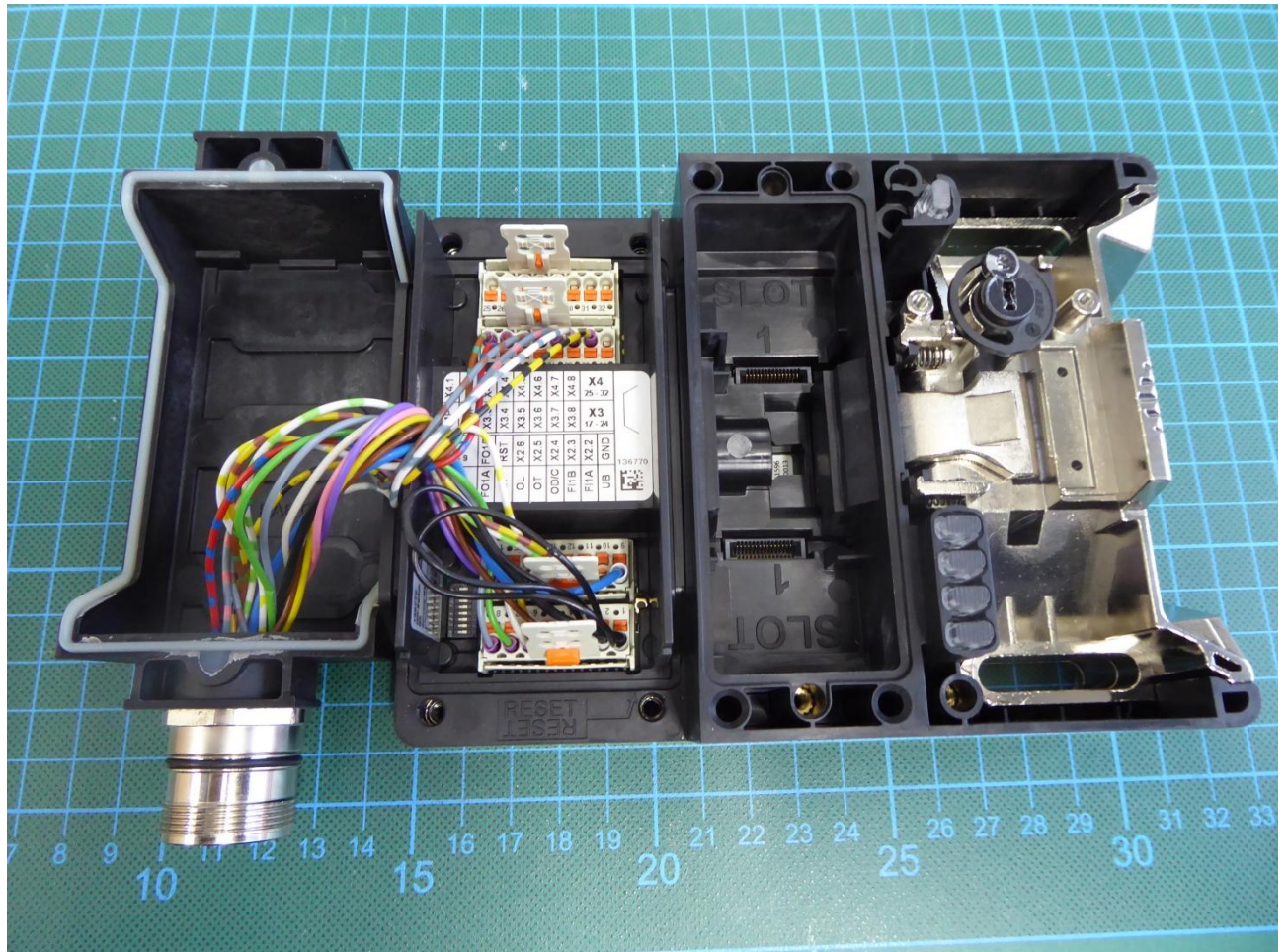
182138_Int7: Front view, cable duct opened
