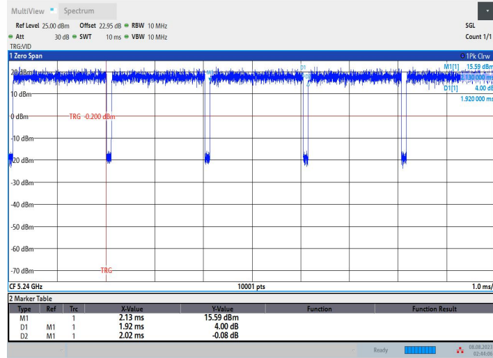
11N20SISO_Ant2_5240
