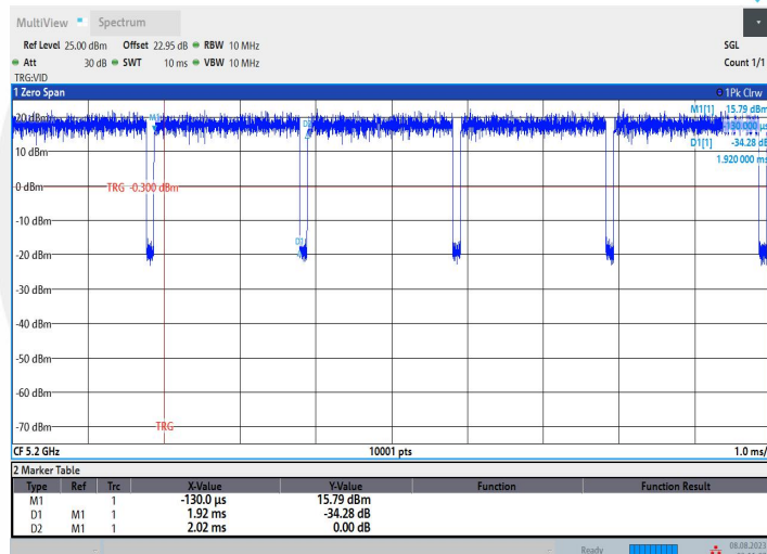
11N20SISO_Ant1_5240
