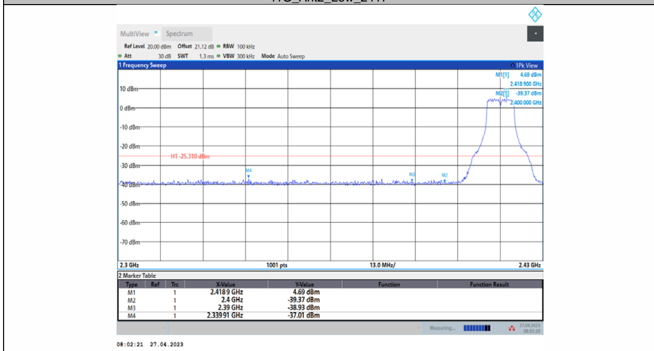
11N20SISO_Ant1_Low_2417
