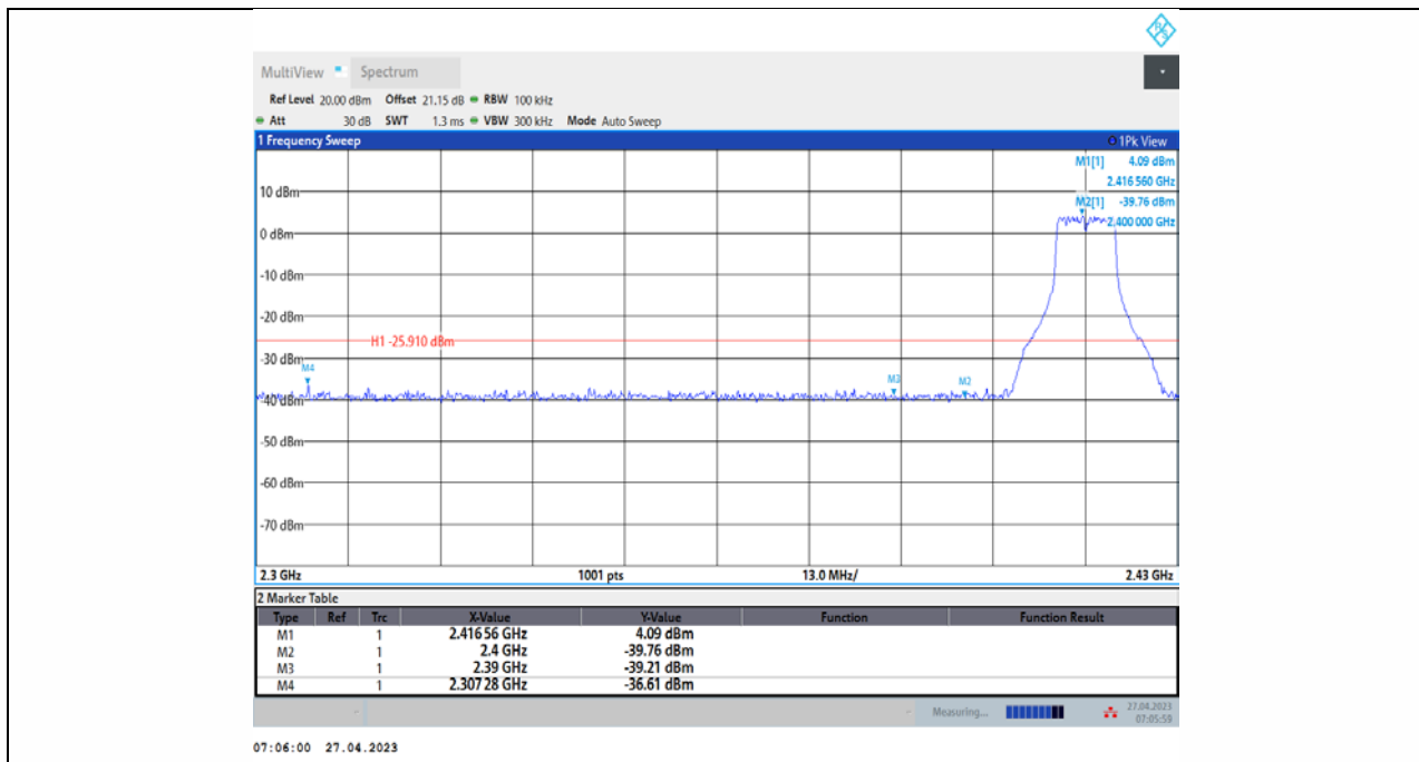
11G_Ant2_Low_2417
