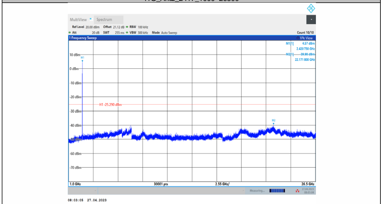
11N20SISO_Ant1_2417_0~Reference
