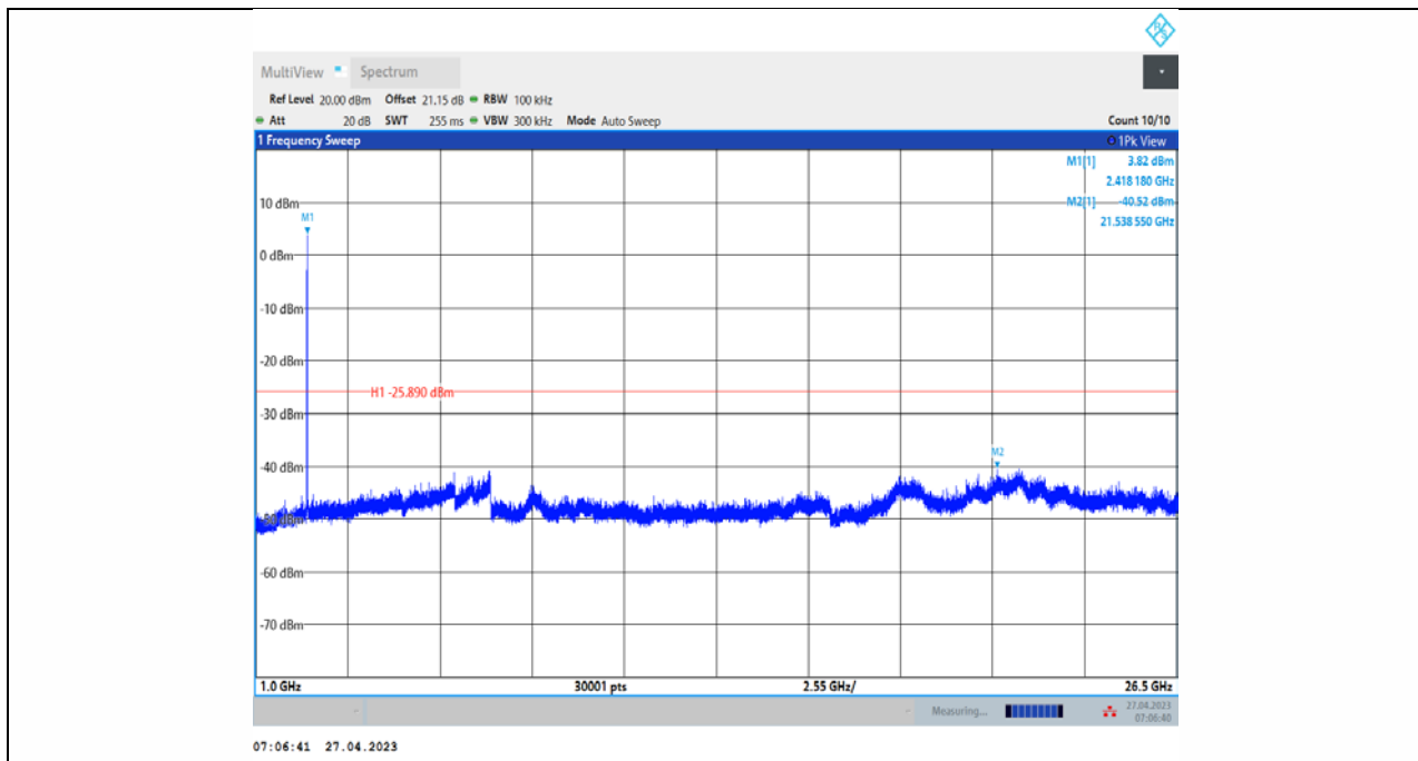
11G_Ant2_2417_0~Reference
