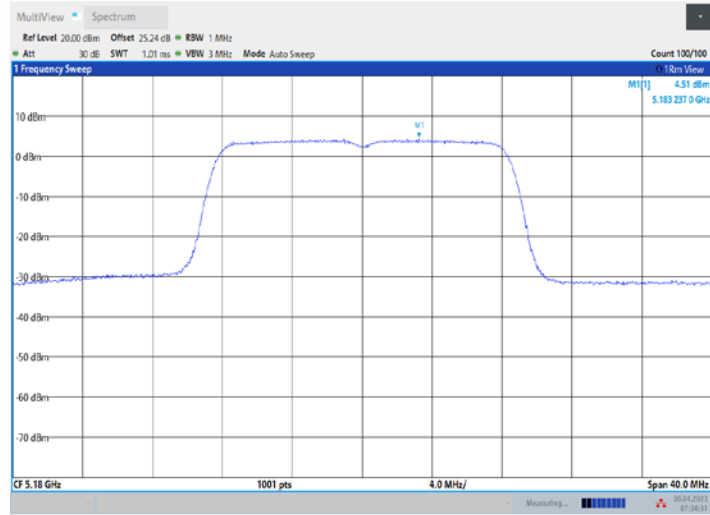
11A_Ant2_5180
