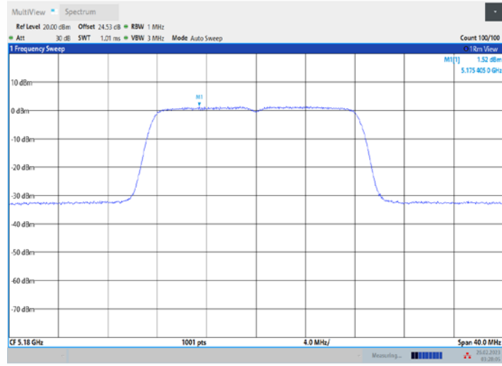
11A_Ant2_5180
