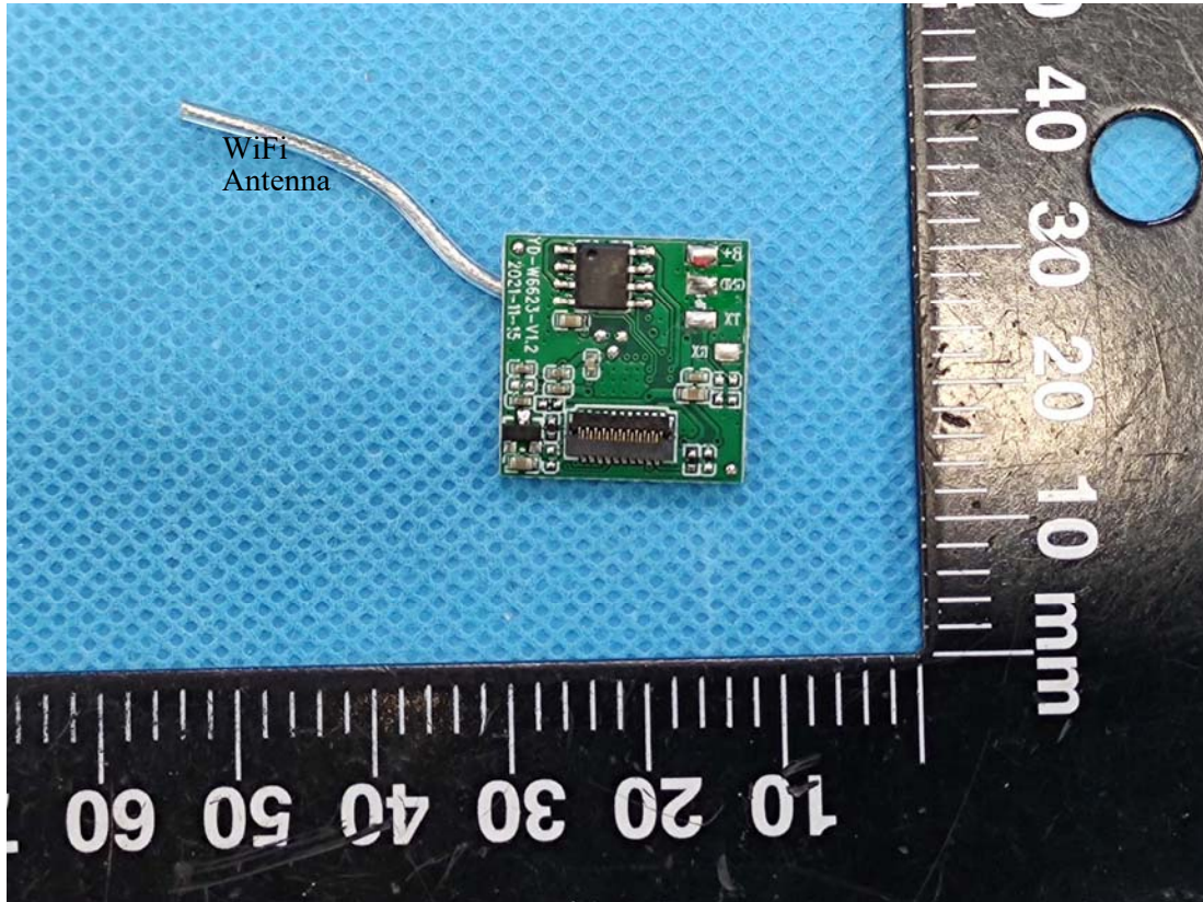
WiFi Board
