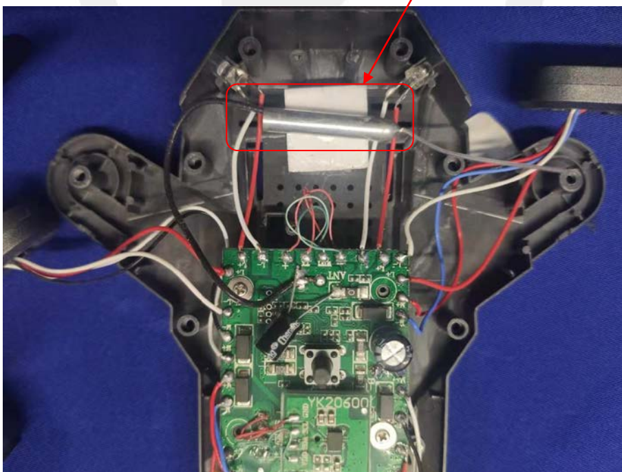
2.4G receiver antenna
